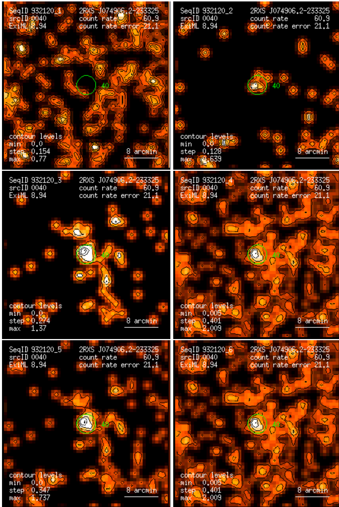
Figure 40: RASS 932120: detection 0040: band rate images, Gaussian filter: (1) PSPC channels 11 – 41, (2) 52 – 90, (3) 91 – 201, (4) 11 – 235, (5) 52 – 201, (6) 11 – 201. Broad band rates in counts/ks. Band rate contour levels in counts/ks/arcmin 2 .
