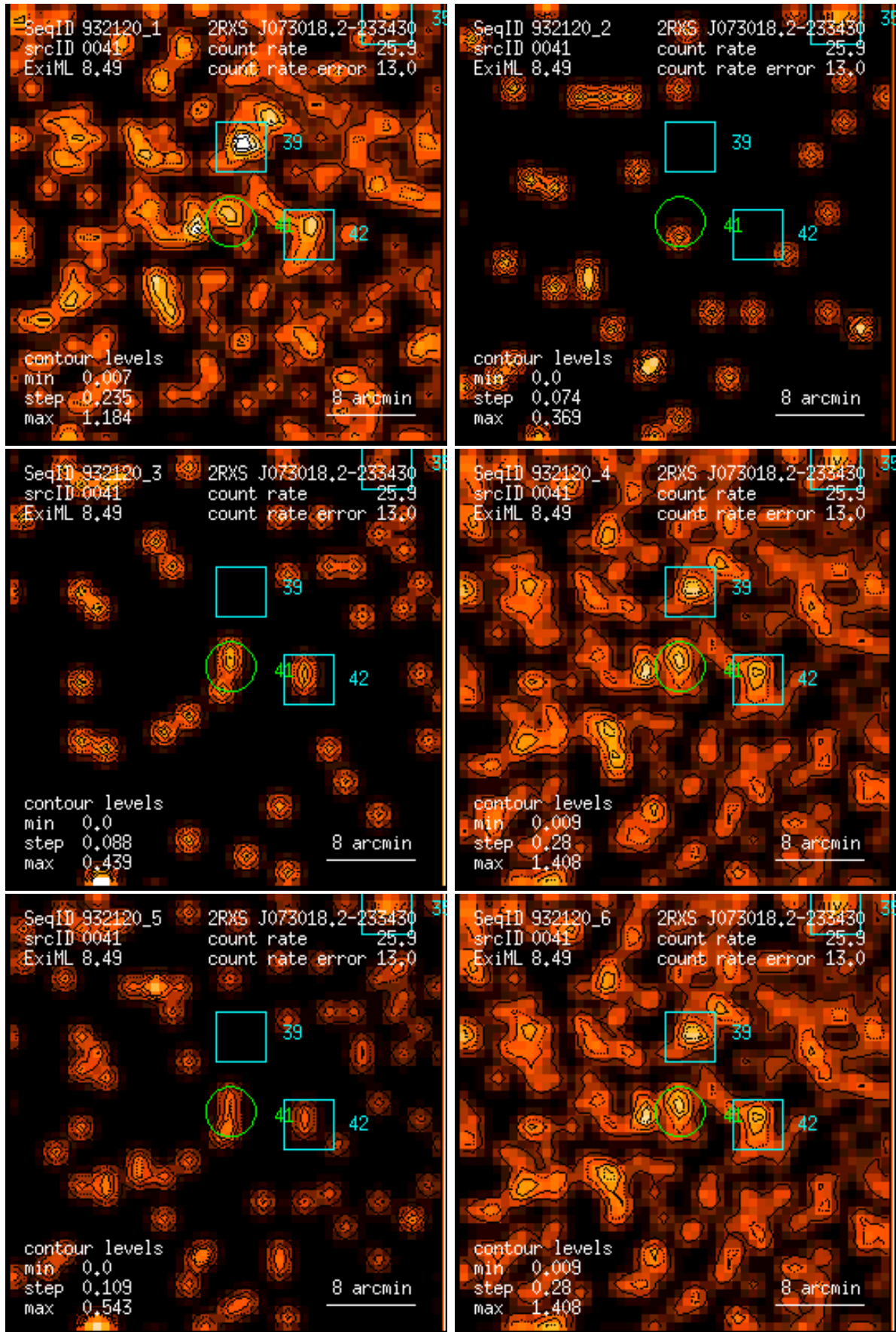
Figure 41: RASS 932120: detection 0041: band rate images, Gaussian filter: (1) PSPC channels 11 – 41, (2) 52 – 90, (3) 91 – 201, (4) 11 – 235, (5) 52 – 201, (6) 11 – 201. Broad band rates in counts/ks. Band rate contour levels in counts/ks/arcmin 2 .
