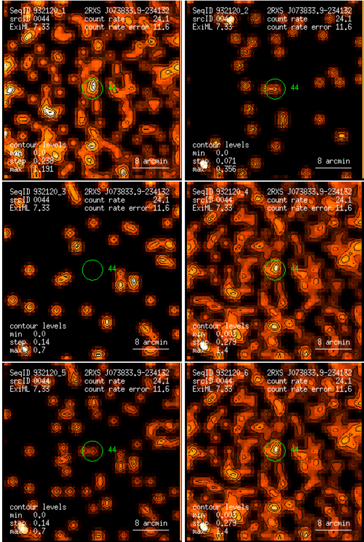
Figure 44: RASS 932120: detection 0044: band rate images, Gaussian filter: (1) PSPC channels 11 – 41, (2) 52 – 90, (3) 91 – 201, (4) 11 – 235, (5) 52 – 201, (6) 11 – 201. Broad band rates in counts/ks. Band rate contour levels in counts/ks/arcmin 2 .
