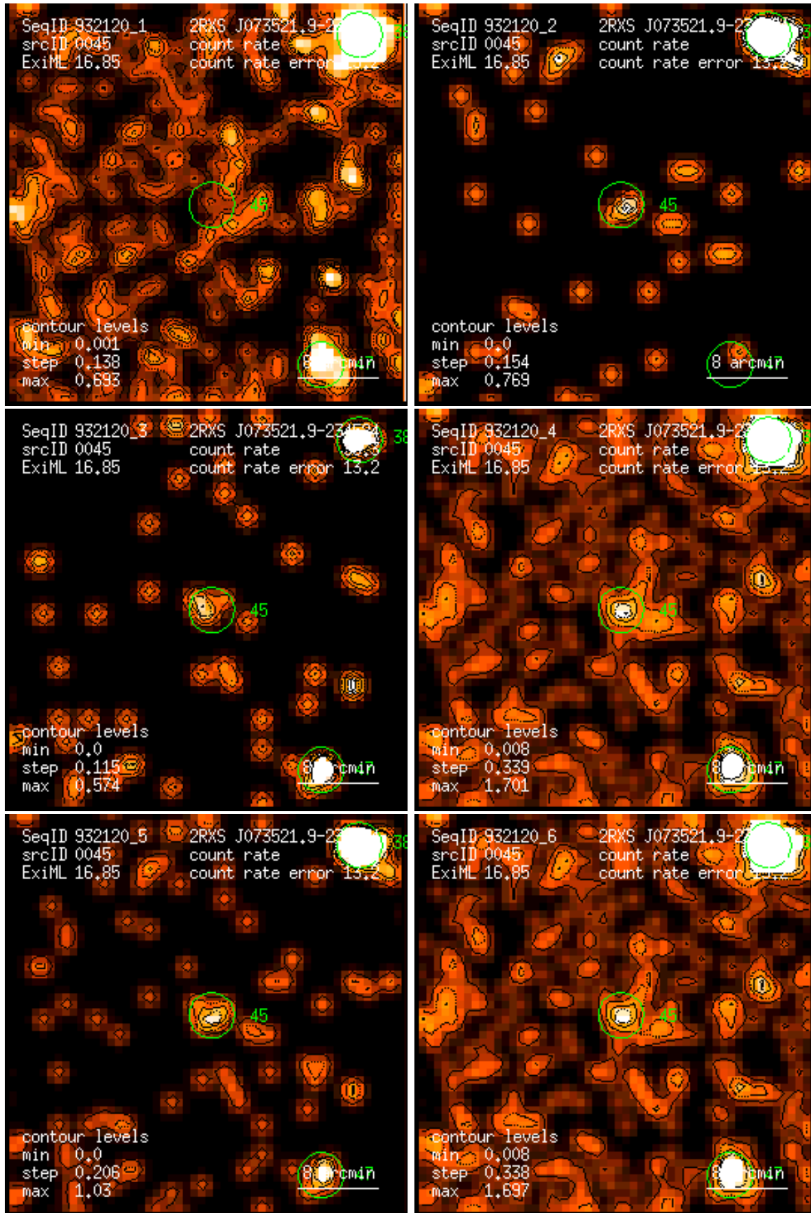
Figure 45: RASS 932120: detection 0045: band rate images, Gaussian filter: (1) PSPC channels 11 – 41, (2) 52 – 90, (3) 91 – 201, (4) 11 – 235, (5) 52 – 201, (6) 11 – 201. Broad band rates in counts/ks. Band rate contour levels in counts/ks/arcmin 2 .
