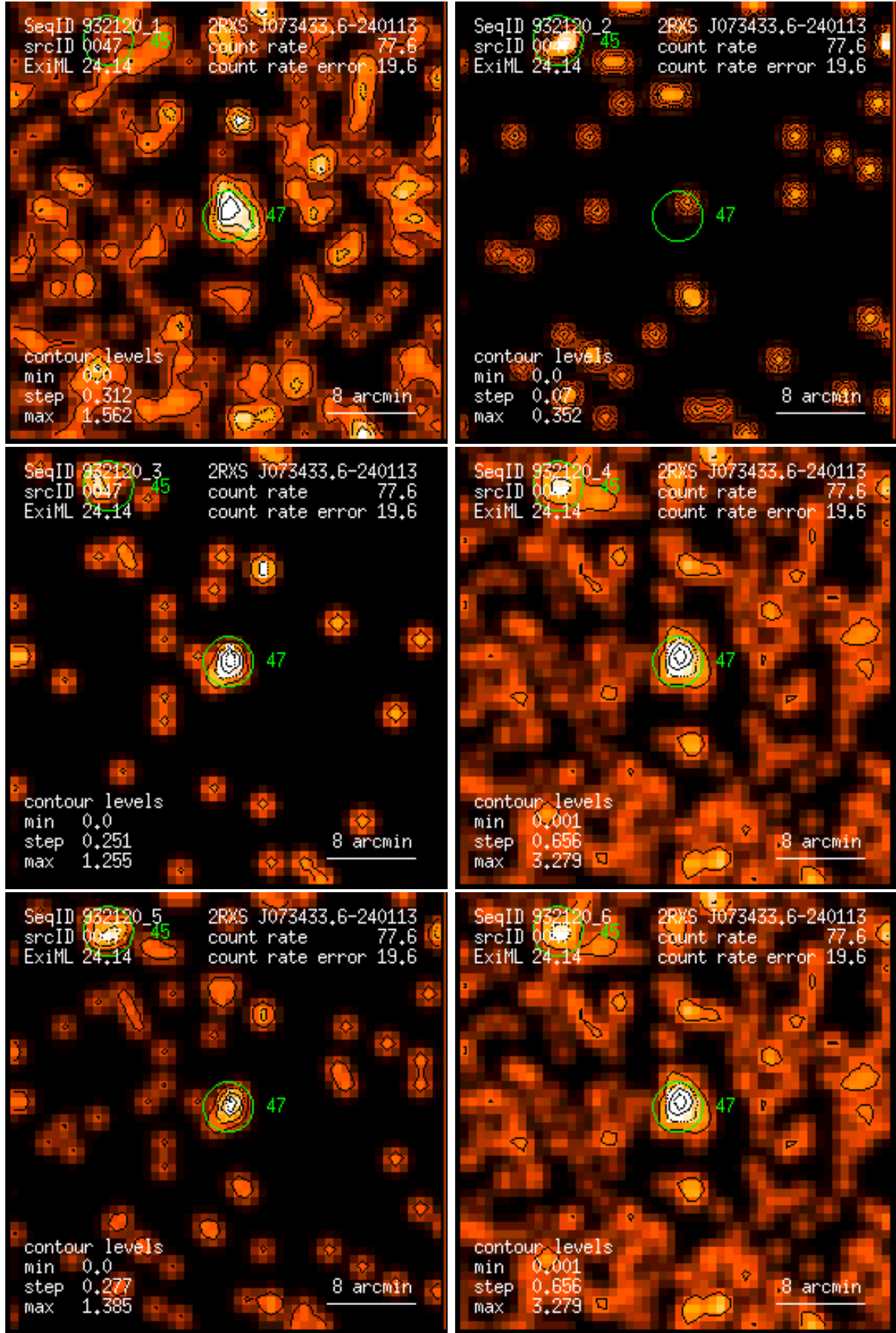
Figure 47: RASS 932120: detection 0047: band rate images, Gaussian filter: (1) PSPC channels 11 – 41, (2) 52 – 90, (3) 91 – 201, (4) 11 – 235, (5) 52 – 201, (6) 11 – 201. Broad band rates in counts/ks. Band rate contour levels in counts/ks/arcmin 2 .
