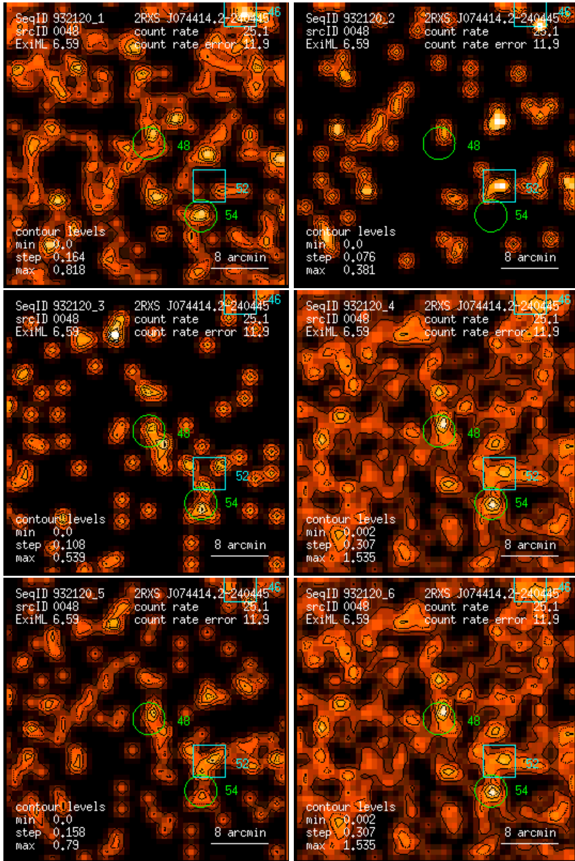
Figure 48: RASS 932120: detection 0048: band rate images, Gaussian filter: (1) PSPC channels 11 – 41, (2) 52 – 90, (3) 91 – 201, (4) 11 – 235, (5) 52 – 201, (6) 11 – 201. Broad band rates in counts/ks. Band rate contour levels in counts/ks/arcmin 2 .
