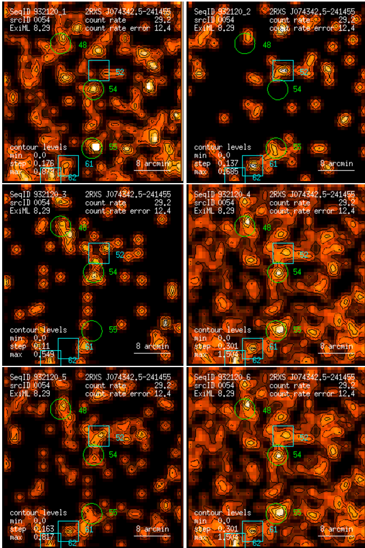
Figure 54: RASS 932120: detection 0054: band rate images, Gaussian filter: (1) PSPC channels 11 – 41, (2) 52 – 90, (3) 91 – 201, (4) 11 – 235, (5) 52 – 201, (6) 11 – 201. Broad band rates in counts/ks. Band rate contour levels in counts/ks/arcmin 2 .
