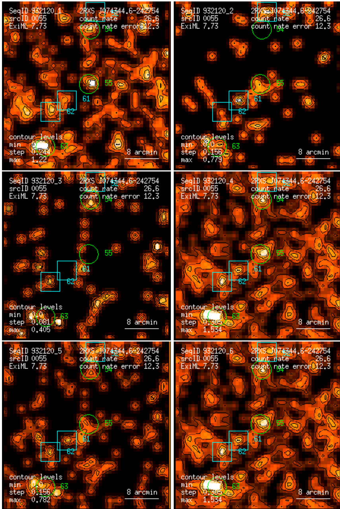
Figure 55: RASS 932120: detection 0055: band rate images, Gaussian filter: (1) PSPC channels 11 – 41, (2) 52 – 90, (3) 91 – 201, (4) 11 – 235, (5) 52 – 201, (6) 11 – 201. Broad band rates in counts/ks. Band rate contour levels in counts/ks/arcmin 2 .
