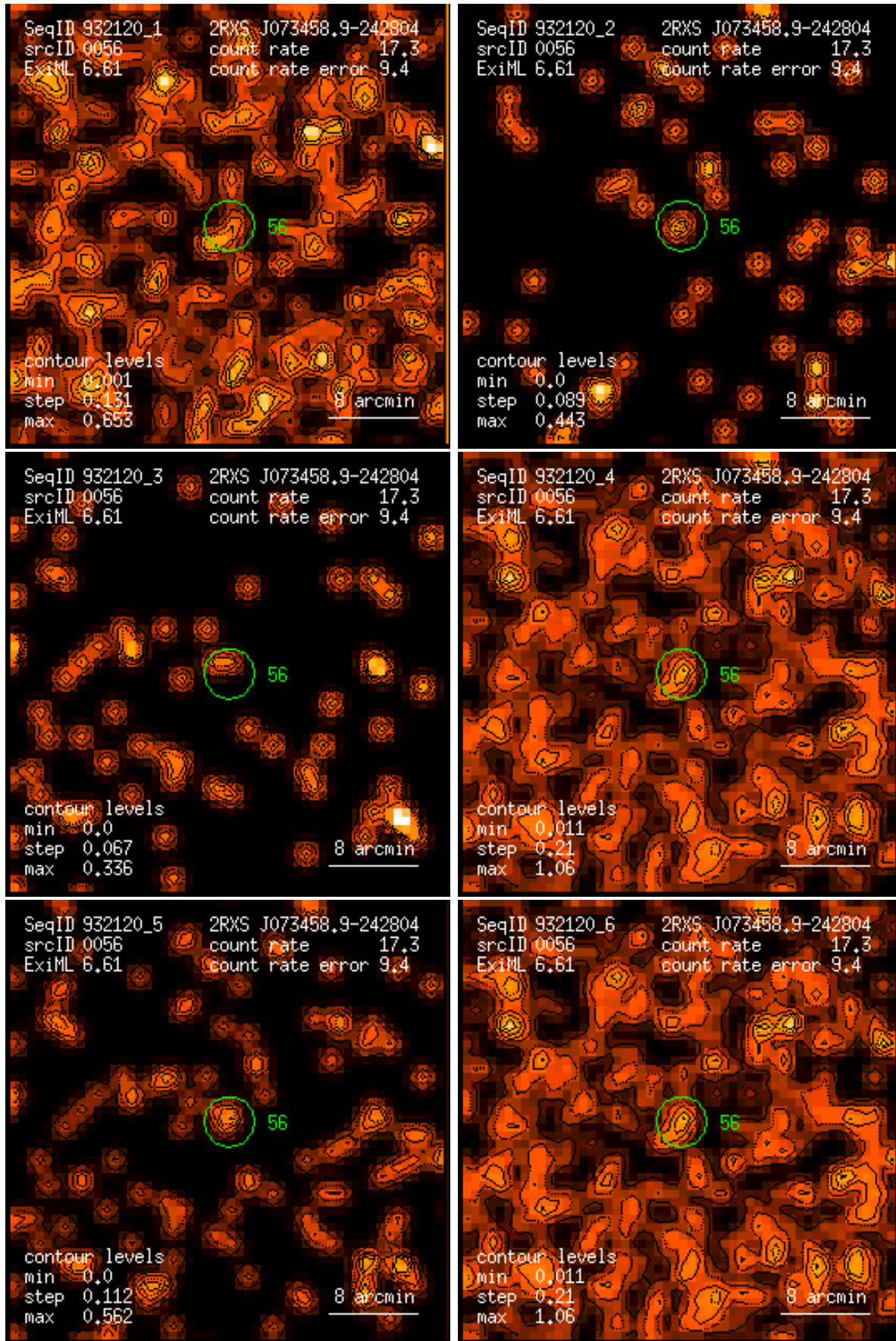
Figure 56: RASS 932120: detection 0056: band rate images, Gaussian filter: (1) PSPC channels 11 – 41, (2) 52 – 90, (3) 91 – 201, (4) 11 – 235, (5) 52 – 201, (6) 11 – 201. Broad band rates in counts/ks. Band rate contour levels in counts/ks/arcmin 2 .
