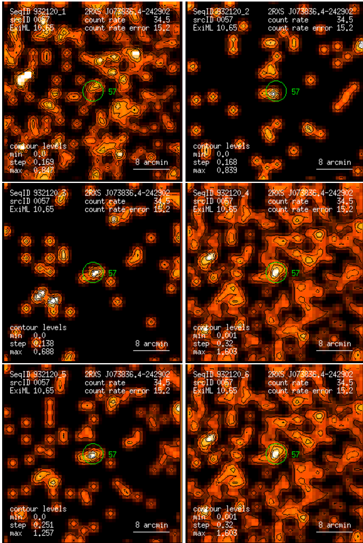
Figure 57: RASS 932120: detection 0057: band rate images, Gaussian filter: (1) PSPC channels 11 – 41, (2) 52 – 90, (3) 91 – 201, (4) 11 – 235, (5) 52 – 201, (6) 11 – 201. Broad band rates in counts/ks. Band rate contour levels in counts/ks/arcmin 2 .
