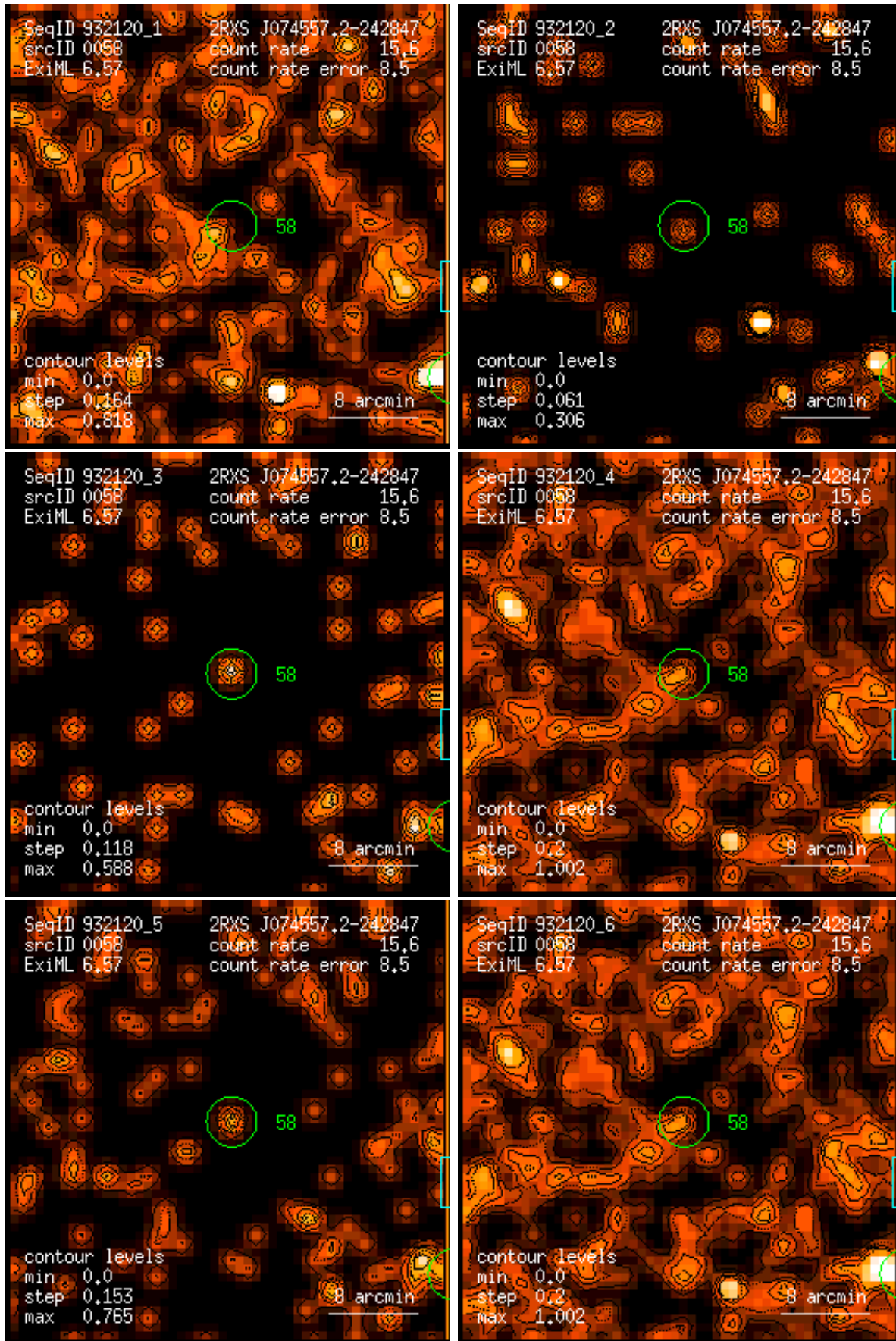
Figure 58: RASS 932120: detection 0058: band rate images, Gaussian filter: (1) PSPC channels 11 – 41, (2) 52 – 90, (3) 91 – 201, (4) 11 – 235, (5) 52 – 201, (6) 11 – 201. Broad band rates in counts/ks. Band rate contour levels in counts/ks/arcmin 2 .
