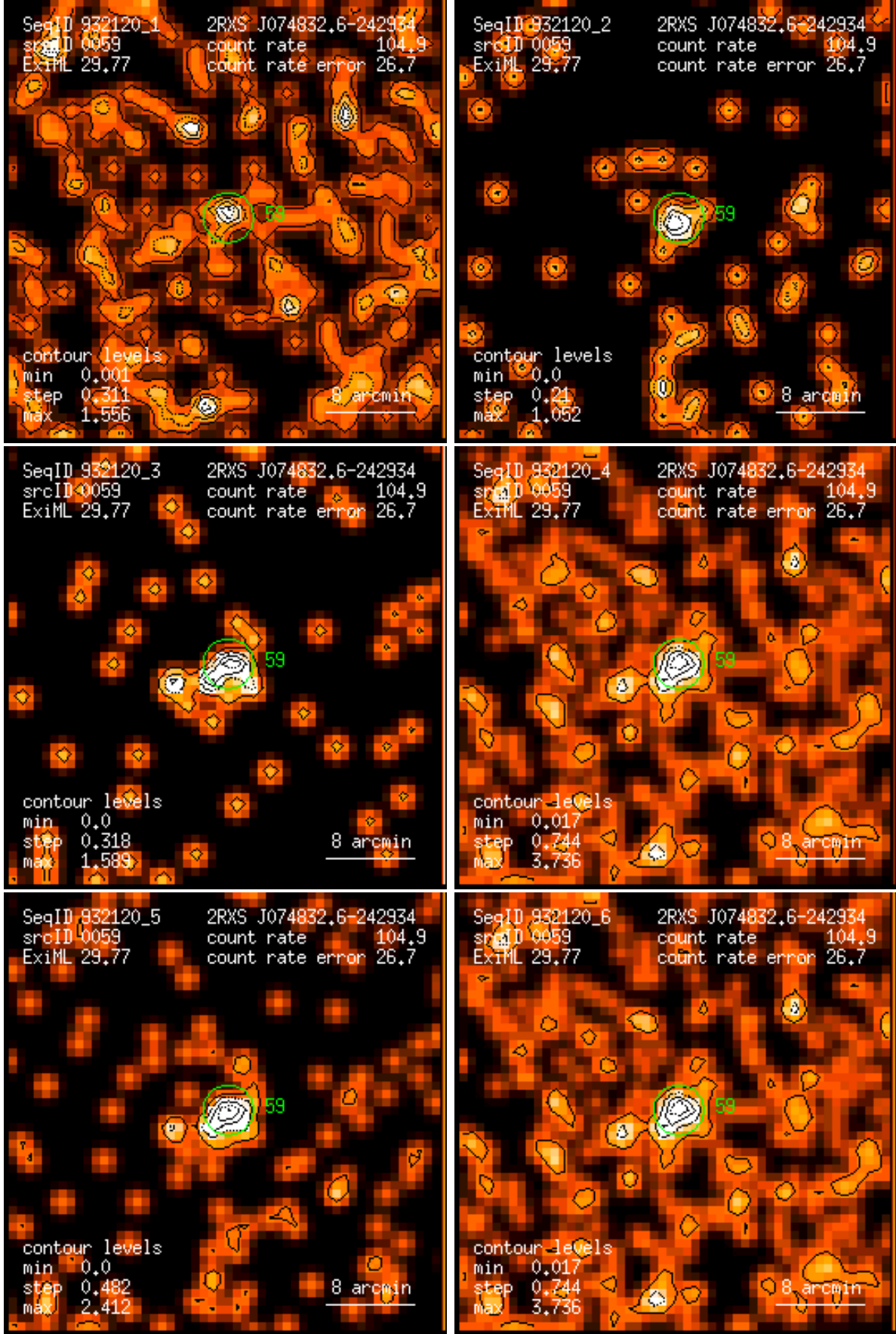
Figure 59: RASS 932120: detection 0059: band rate images, Gaussian filter: (1) PSPC channels 11 – 41, (2) 52 – 90, (3) 91 – 201, (4) 11 – 235, (5) 52 – 201, (6) 11 – 201. Broad band rates in counts/ks. Band rate contour levels in counts/ks/arcmin 2 .
