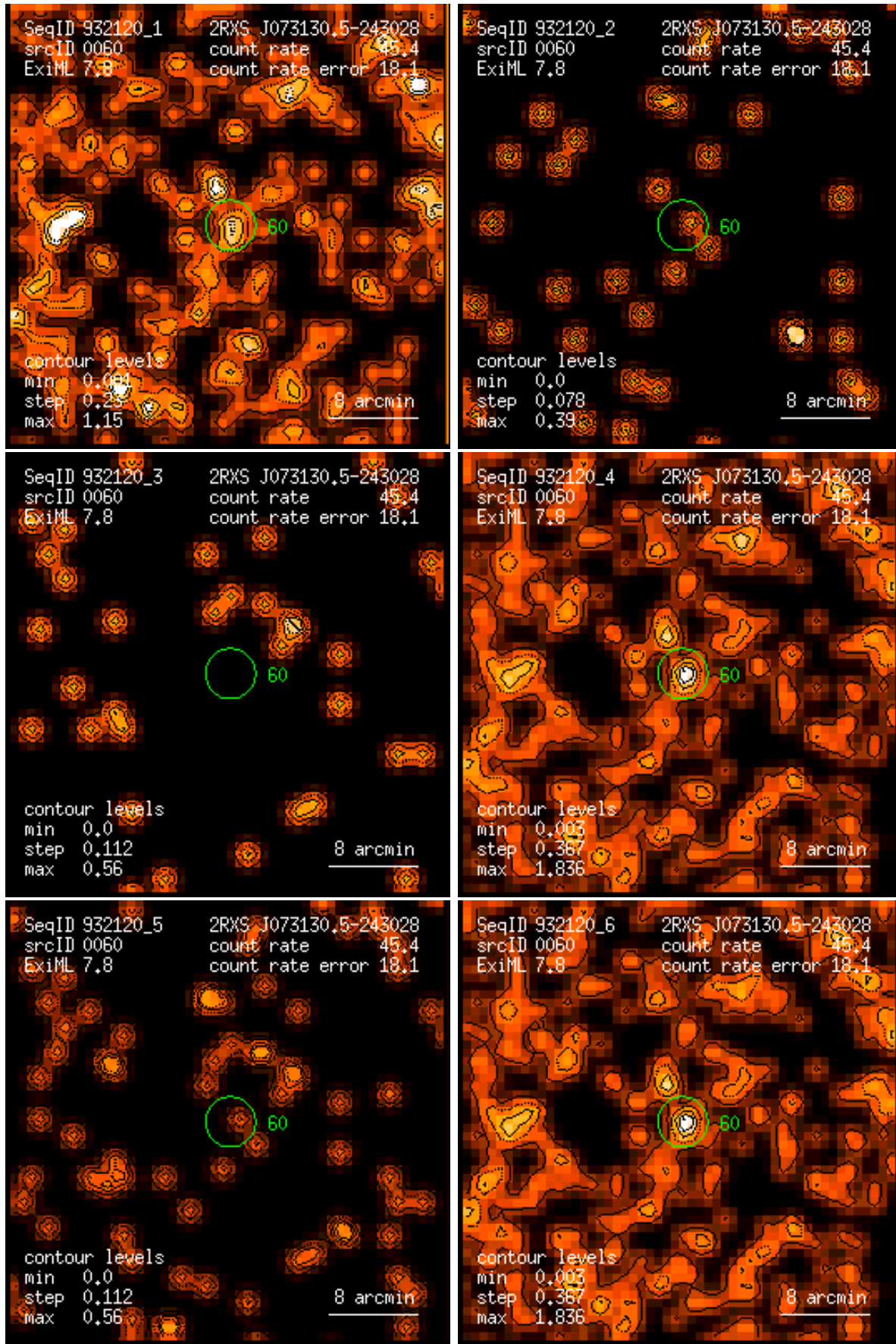
Figure 60: RASS 932120: detection 0060: band rate images, Gaussian filter: (1) PSPC channels 11 – 41, (2) 52 – 90, (3) 91 – 201, (4) 11 – 235, (5) 52 – 201, (6) 11 – 201. Broad band rates in counts/ks. Band rate contour levels in counts/ks/arcmin 2 .
