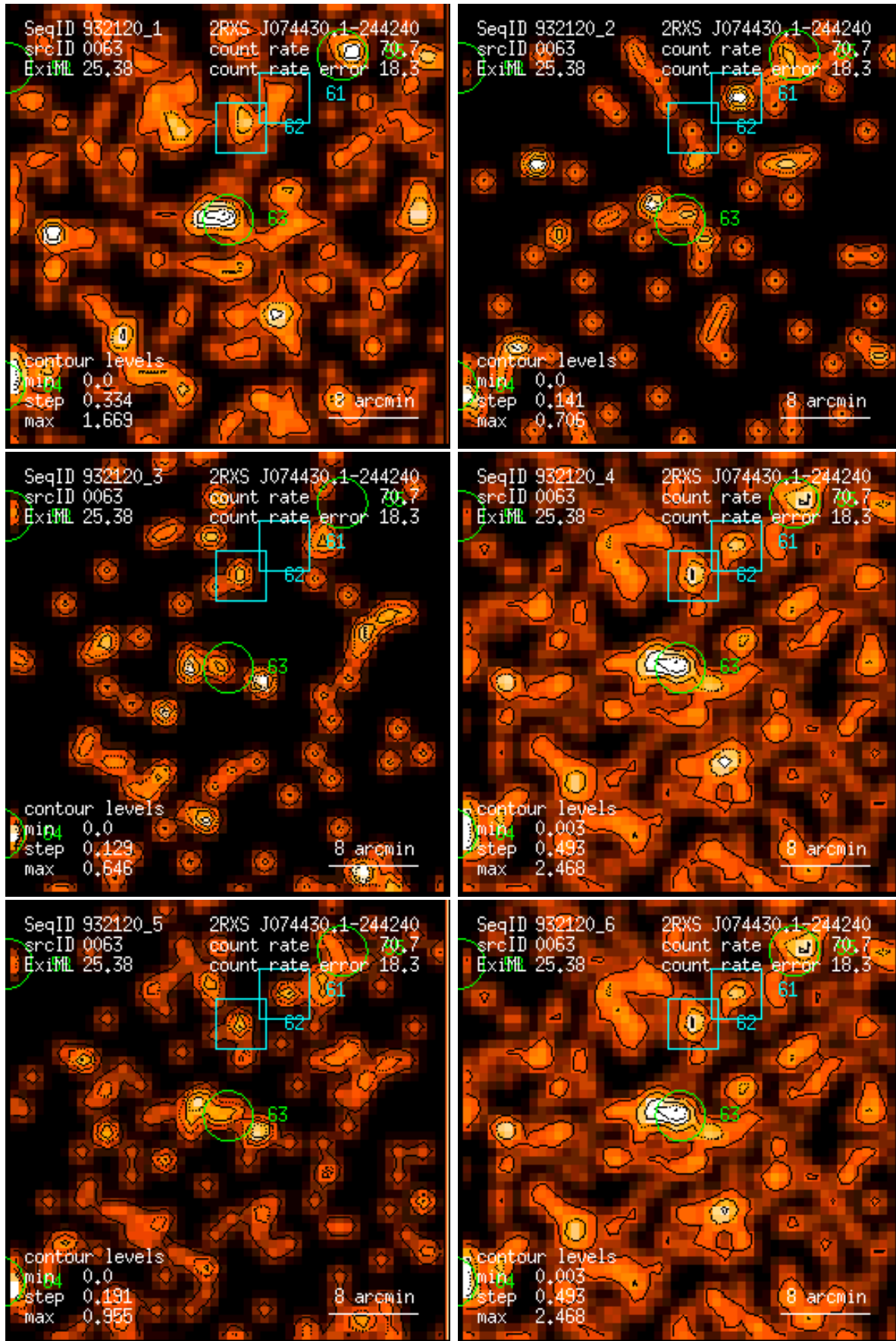
Figure 63: RASS 932120: detection 0063: band rate images, Gaussian filter: (1) PSPC channels 11 – 41, (2) 52 – 90, (3) 91 – 201, (4) 11 – 235, (5) 52 – 201, (6) 11 – 201. Broad band rates in counts/ks. Band rate contour levels in counts/ks/arcmin 2 .
