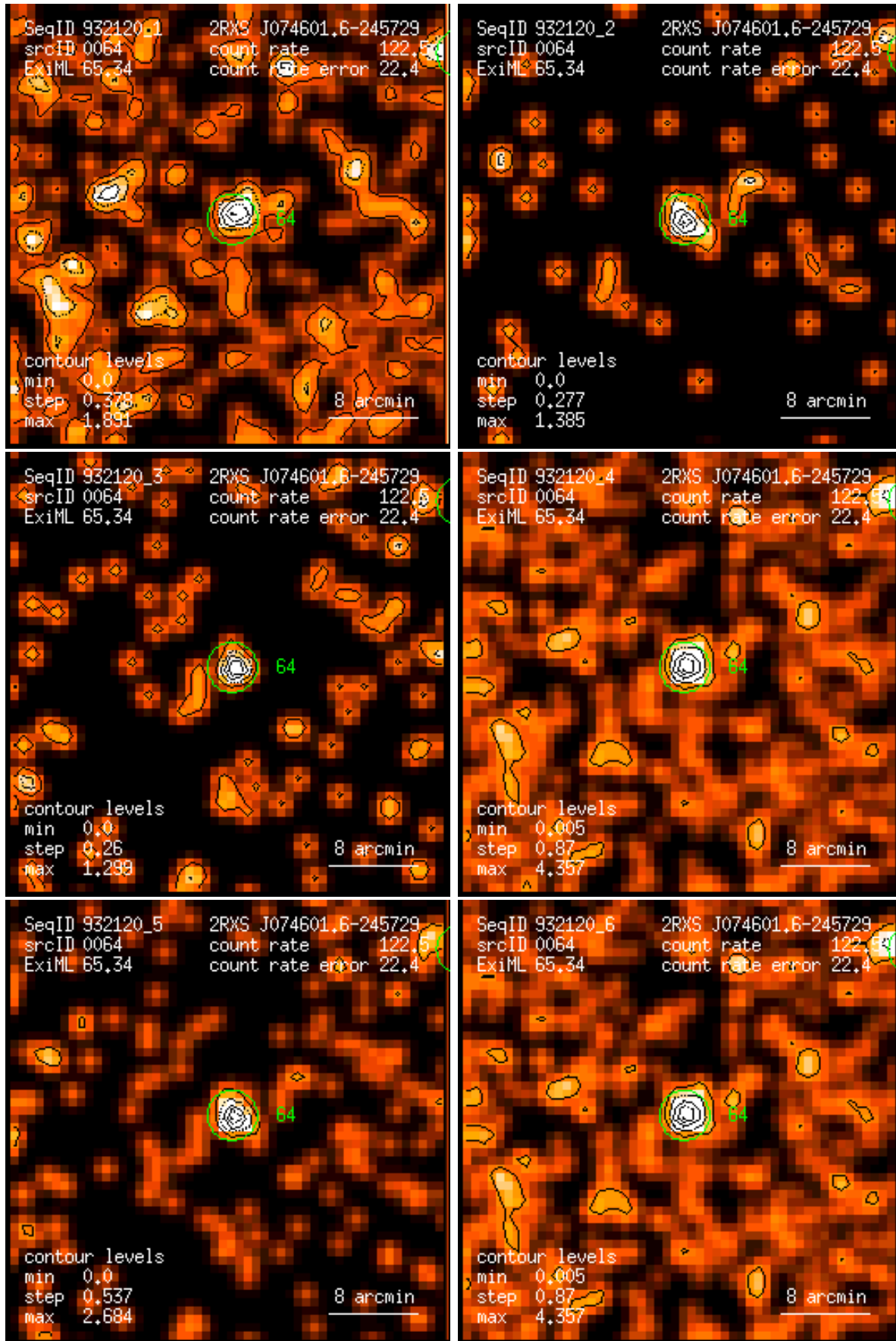
Figure 64: RASS 932120: detection 0064: band rate images, Gaussian filter: (1) PSPC channels 11 – 41, (2) 52 – 90, (3) 91 – 201, (4) 11 – 235, (5) 52 – 201, (6) 11 – 201. Broad band rates in counts/ks. Band rate contour levels in counts/ks/arcmin 2 .
