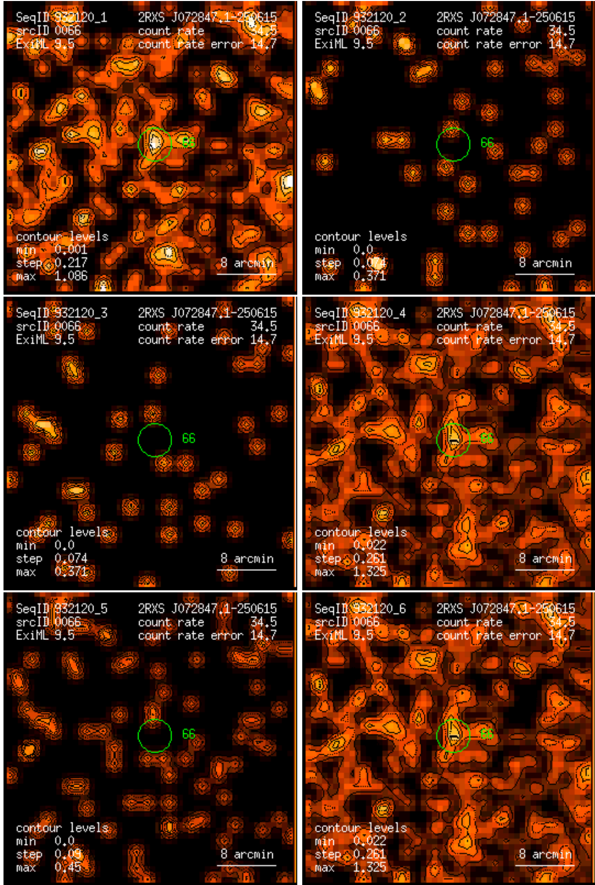
Figure 66: RASS 932120: detection 0066: band rate images, Gaussian filter: (1) PSPC channels 11 – 41, (2) 52 – 90, (3) 91 – 201, (4) 11 – 235, (5) 52 – 201, (6) 11 – 201. Broad band rates in counts/ks. Band rate contour levels in counts/ks/arcmin 2 .
