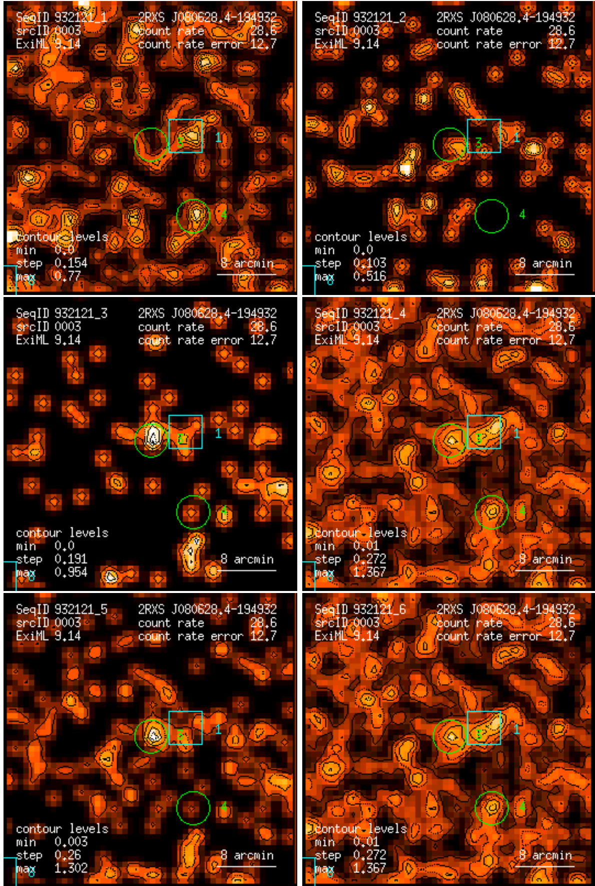
Figure 3: RASS 932121: detection 0003: band rate images, Gaussian filter: (1) PSPC channels 11 – 41, (2) 52 – 90, (3) 91 – 201, (4) 11 – 235, (5) 52 – 201, (6) 11 – 201. Broad band rates in counts/ks. Band rate contour levels in counts/ks/arcmin 2 .
