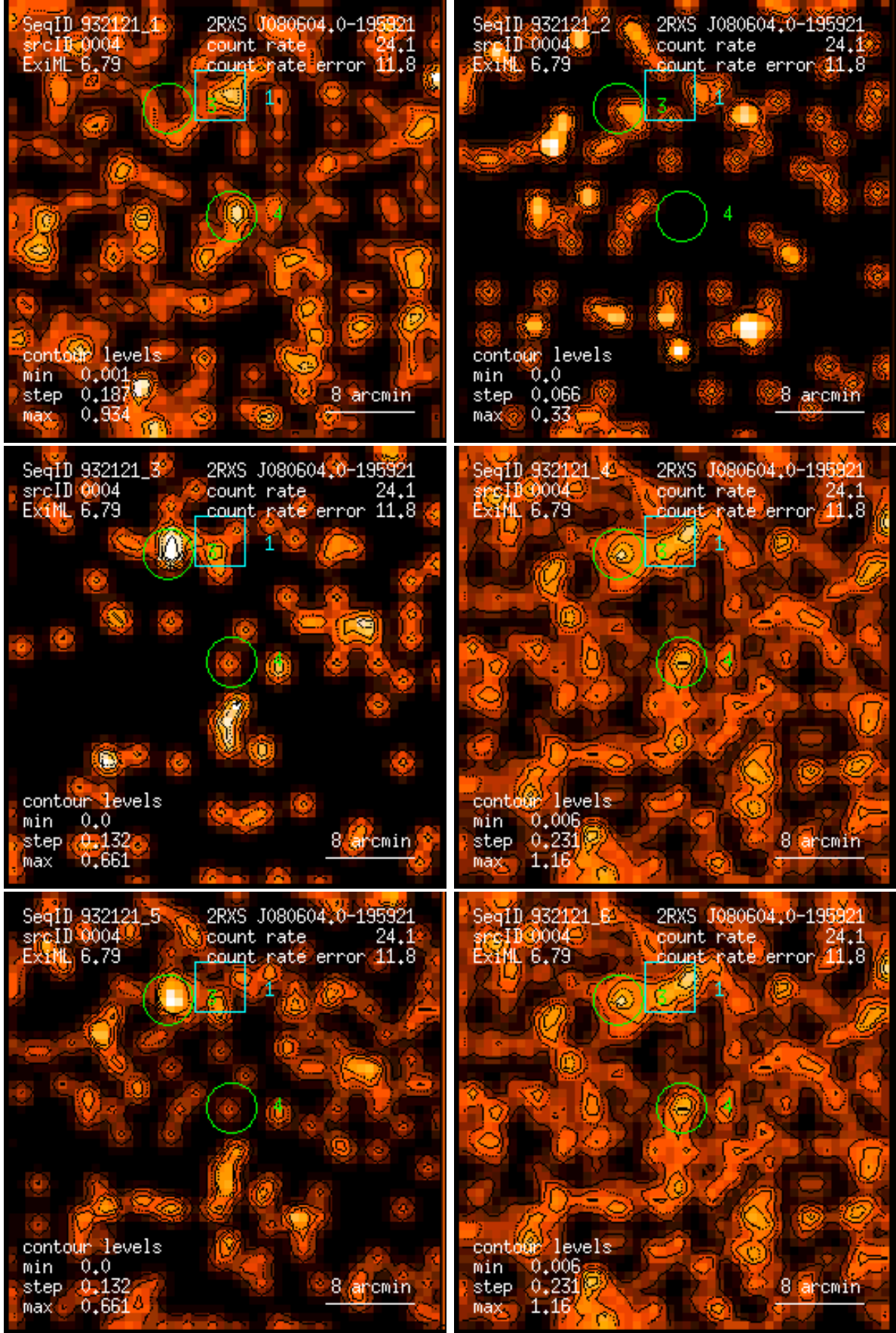
Figure 4: RASS 932121: detection 0004: band rate images, Gaussian filter: (1) PSPC channels 11 – 41, (2) 52 – 90, (3) 91 – 201, (4) 11 – 235, (5) 52 – 201, (6) 11 – 201. Broad band rates in counts/ks. Band rate contour levels in counts/ks/arcmin 2 .
