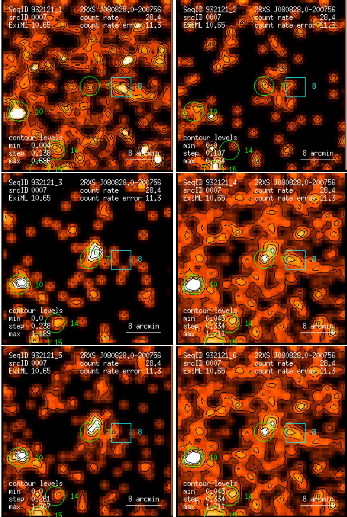
Figure 7: RASS 932121: detection 0007: band rate images, Gaussian filter: (1) PSPC channels 11 – 41, (2) 52 – 90, (3) 91 – 201, (4) 11 – 235, (5) 52 – 201, (6) 11 – 201. Broad band rates in counts/ks. Band rate contour levels in counts/ks/arcmin 2 .
