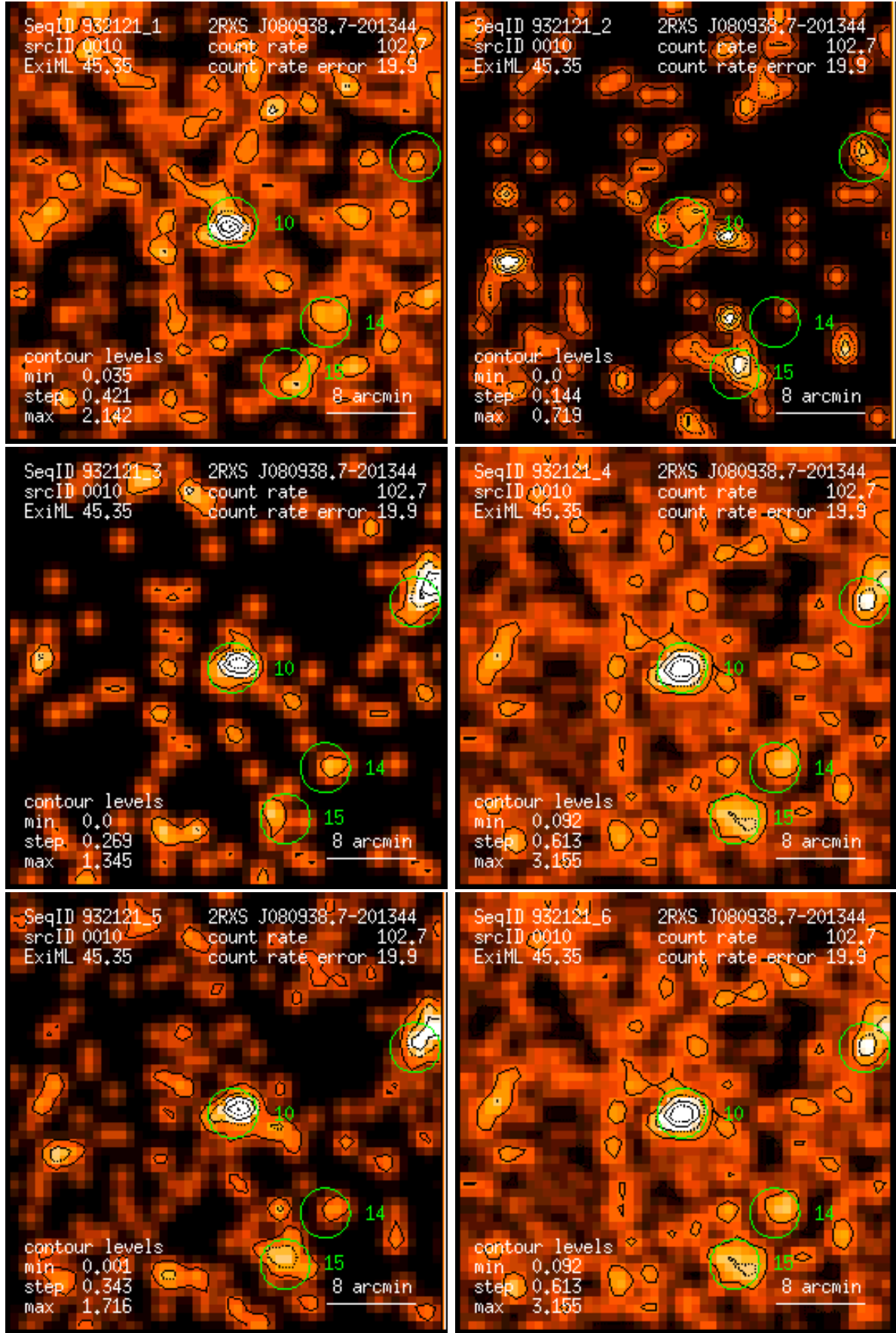
Figure 10: RASS 932121: detection 0010: band rate images, Gaussian filter: (1) PSPC channels 11 – 41, (2) 52 – 90, (3) 91 – 201, (4) 11 – 235, (5) 52 – 201, (6) 11 – 201. Broad band rates in counts/ks. Band rate contour levels in counts/ks/arcmin 2 .
