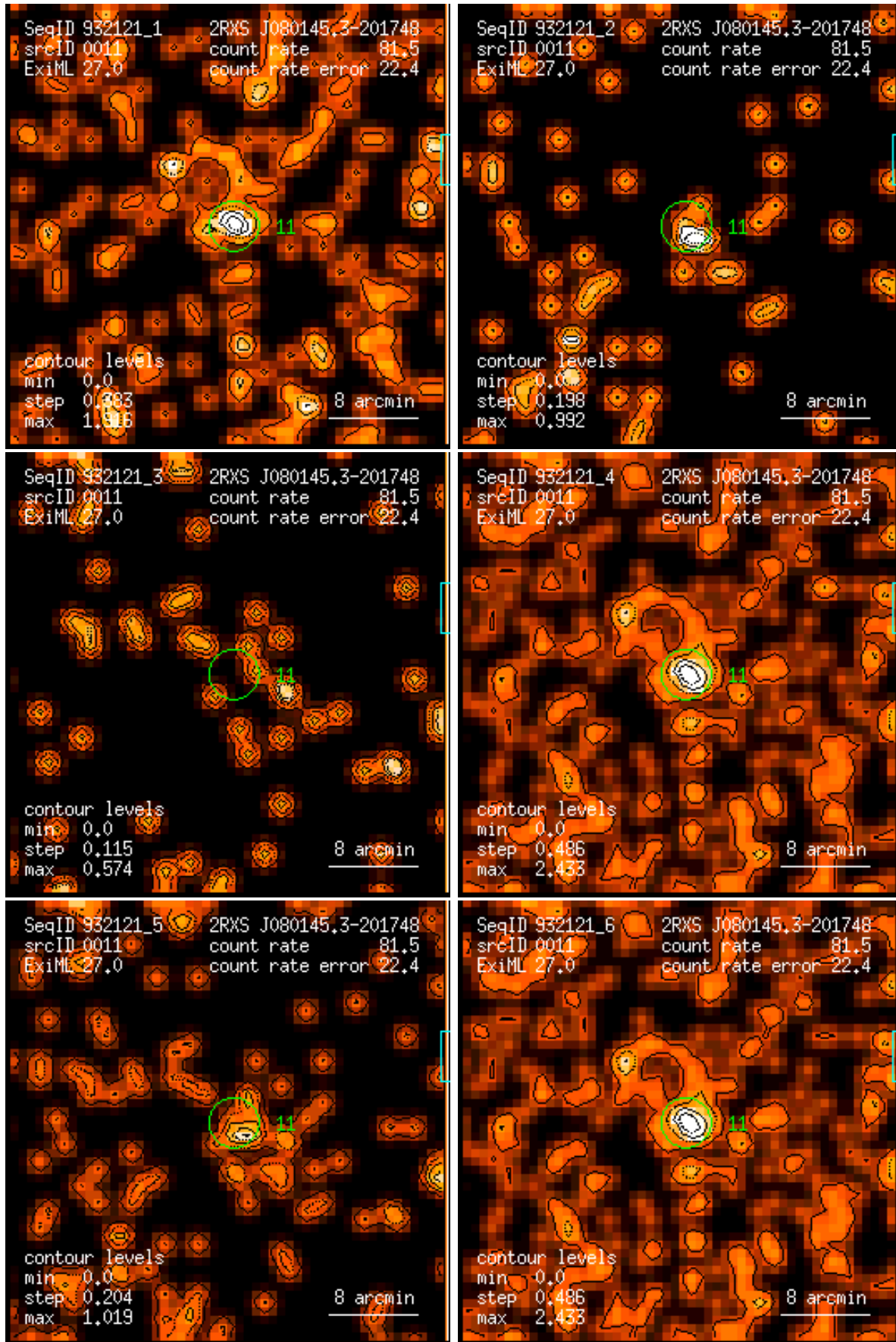
Figure 11: RASS 932121: detection 0011: band rate images, Gaussian filter: (1) PSPC channels 11 – 41, (2) 52 – 90, (3) 91 – 201, (4) 11 – 235, (5) 52 – 201, (6) 11 – 201. Broad band rates in counts/ks. Band rate contour levels in counts/ks/arcmin 2 .
