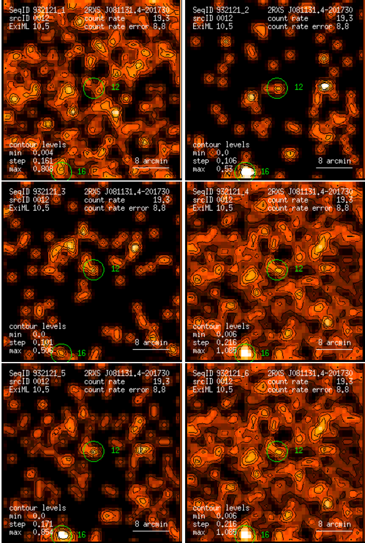
Figure 12: RASS 932121: detection 0012: band rate images, Gaussian filter: (1) PSPC channels 11 – 41, (2) 52 – 90, (3) 91 – 201, (4) 11 – 235, (5) 52 – 201, (6) 11 – 201. Broad band rates in counts/ks. Band rate contour levels in counts/ks/arcmin 2 .
