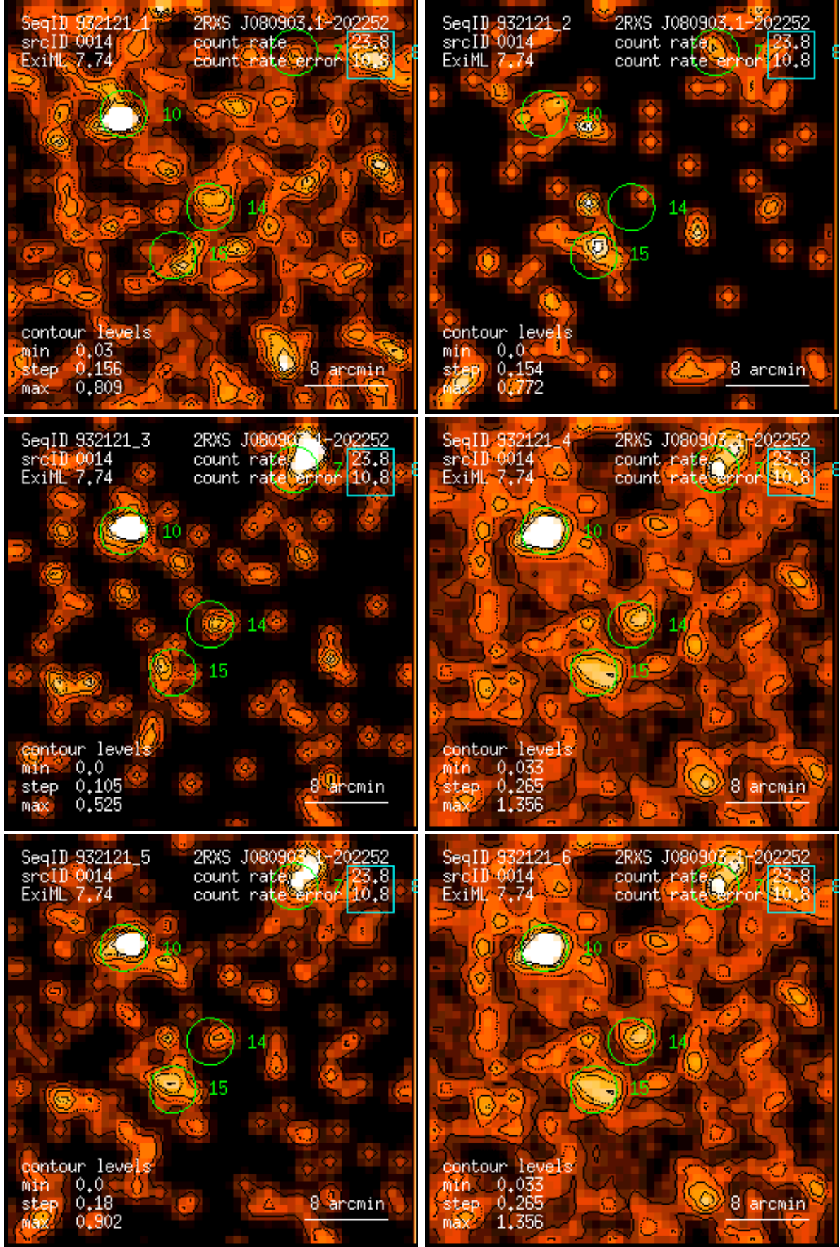
Figure 14: RASS 932121: detection 0014: band rate images, Gaussian filter: (1) PSPC channels 11 – 41, (2) 52 – 90, (3) 91 – 201, (4) 11 – 235, (5) 52 – 201, (6) 11 – 201. Broad band rates in counts/ks. Band rate contour levels in counts/ks/arcmin 2 .
