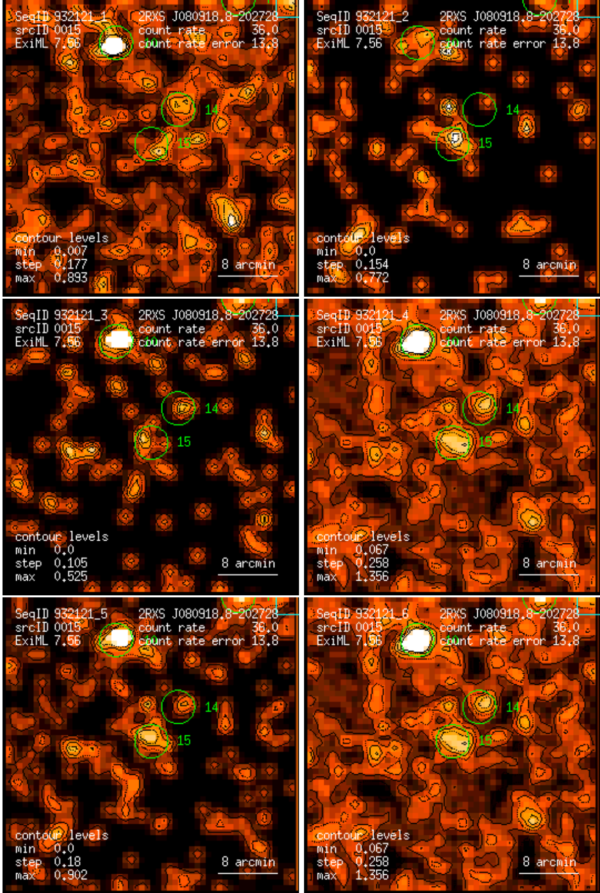
Figure 15: RASS 932121: detection 0015: band rate images, Gaussian filter: (1) PSPC channels 11 – 41, (2) 52 – 90, (3) 91 – 201, (4) 11 – 235, (5) 52 – 201, (6) 11 – 201. Broad band rates in counts/ks. Band rate contour levels in counts/ks/arcmin 2 .
