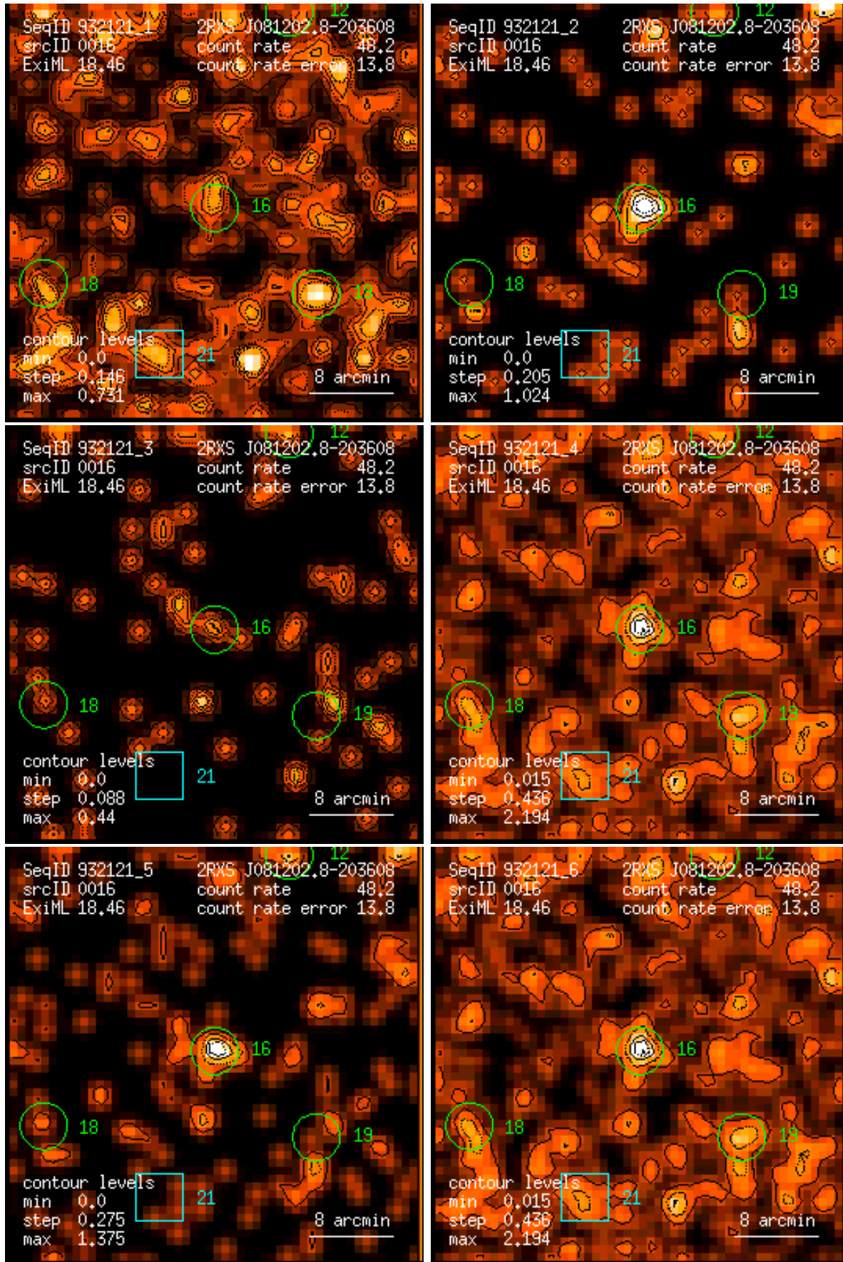
Figure 16: RASS 932121: detection 0016: band rate images, Gaussian filter: (1) PSPC channels 11 – 41, (2) 52 – 90, (3) 91 – 201, (4) 11 – 235, (5) 52 – 201, (6) 11 – 201. Broad band rates in counts/ks. Band rate contour levels in counts/ks/arcmin 2 .
