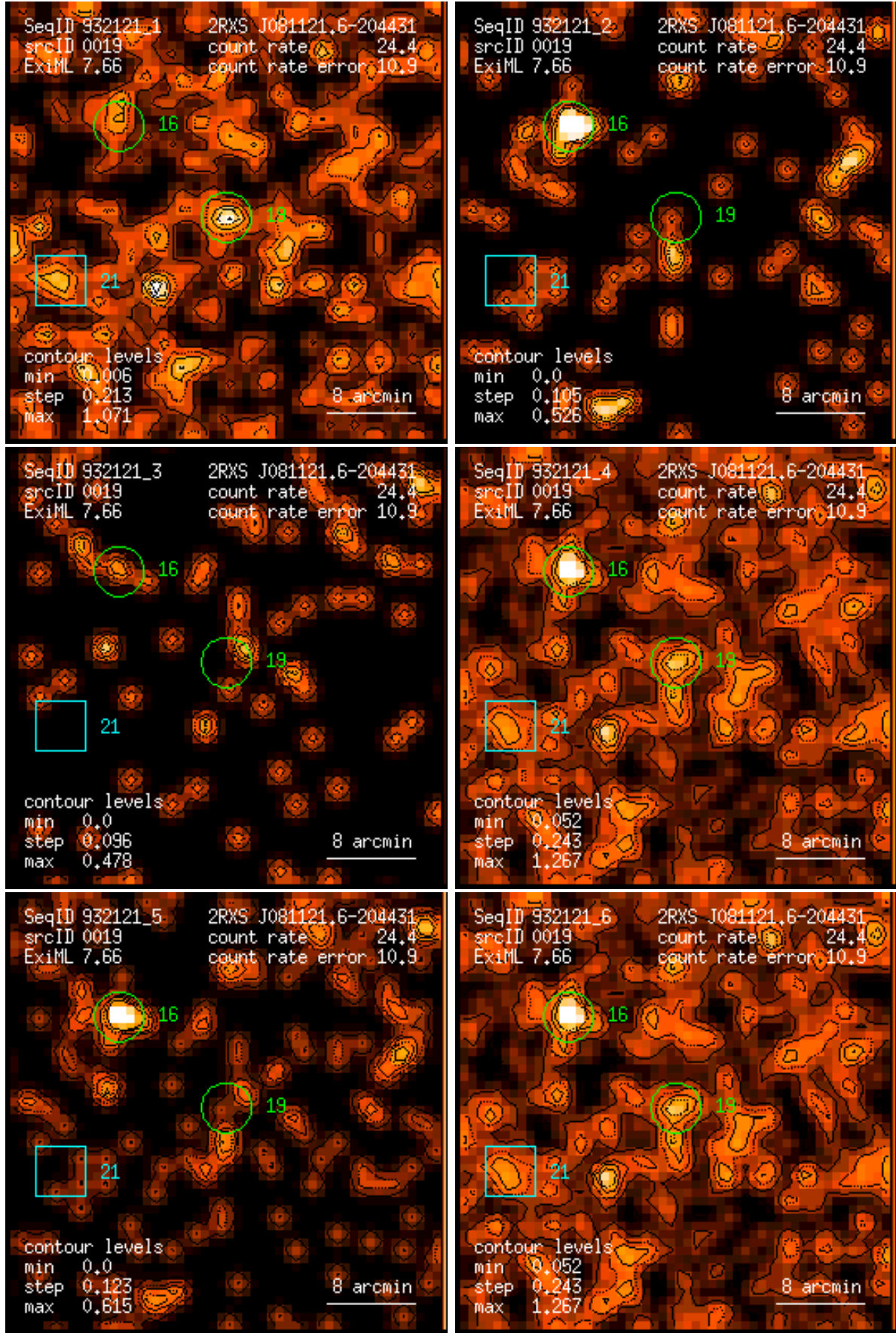
Figure 19: RASS 932121: detection 0019: band rate images, Gaussian filter: (1) PSPC channels 11 – 41, (2) 52 – 90, (3) 91 – 201, (4) 11 – 235, (5) 52 – 201, (6) 11 – 201. Broad band rates in counts/ks. Band rate contour levels in counts/ks/arcmin 2 .
