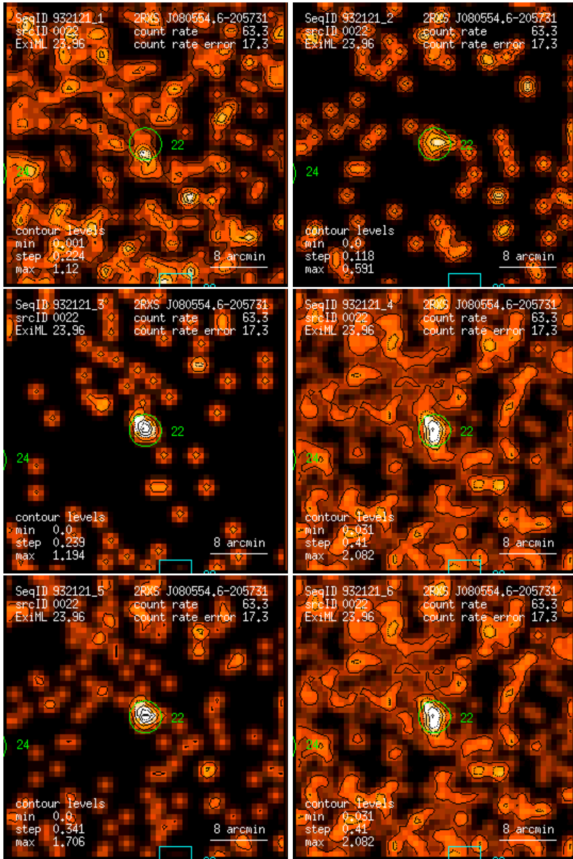
Figure 22: RASS 932121: detection 0022: band rate images, Gaussian filter: (1) PSPC channels 11 – 41, (2) 52 – 90, (3) 91 – 201, (4) 11 – 235, (5) 52 – 201, (6) 11 – 201. Broad band rates in counts/ks. Band rate contour levels in counts/ks/arcmin 2 .
