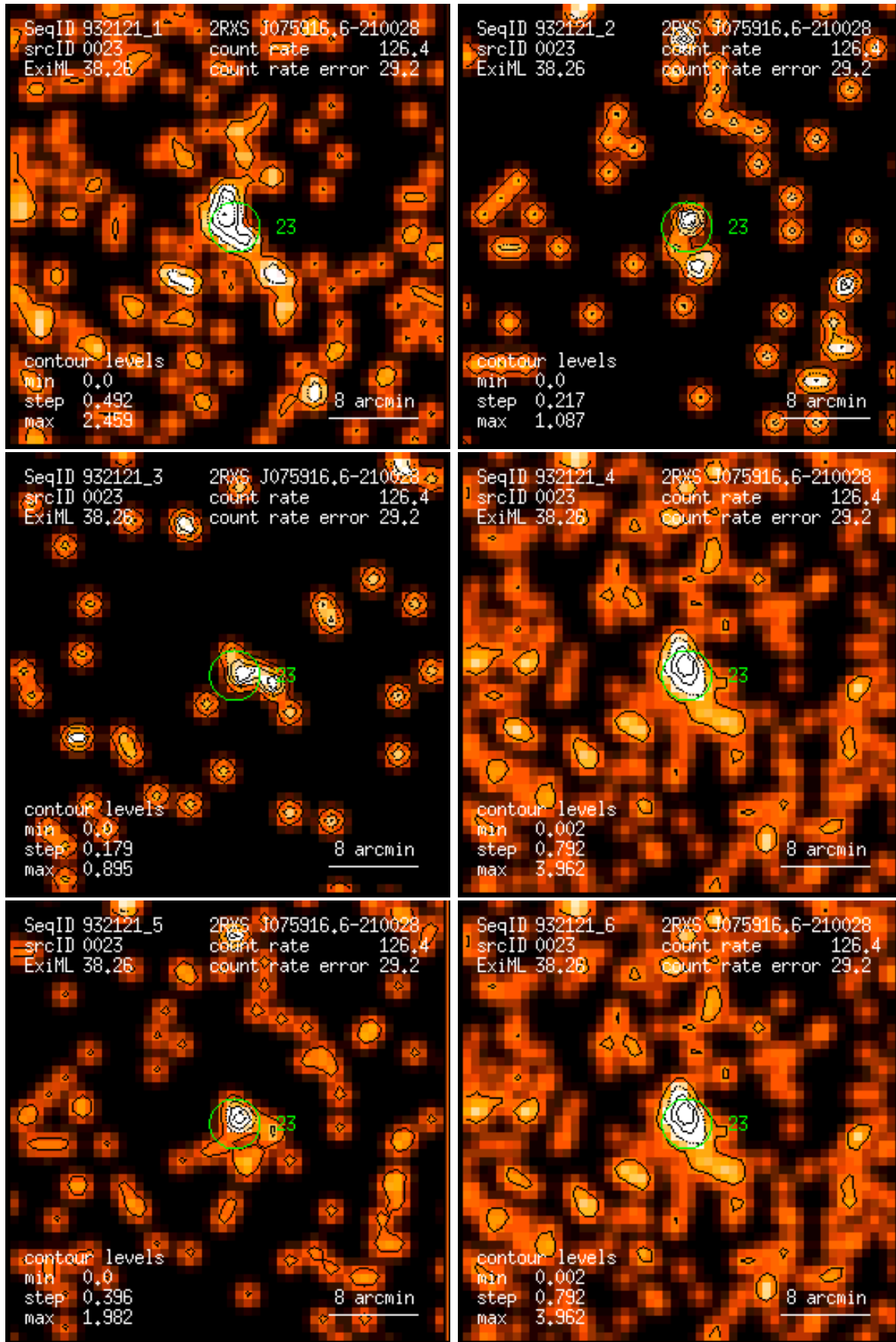
Figure 23: RASS 932121: detection 0023: band rate images, Gaussian filter: (1) PSPC channels 11 – 41, (2) 52 – 90, (3) 91 – 201, (4) 11 – 235, (5) 52 – 201, (6) 11 – 201. Broad band rates in counts/ks. Band rate contour levels in counts/ks/arcmin 2 .
