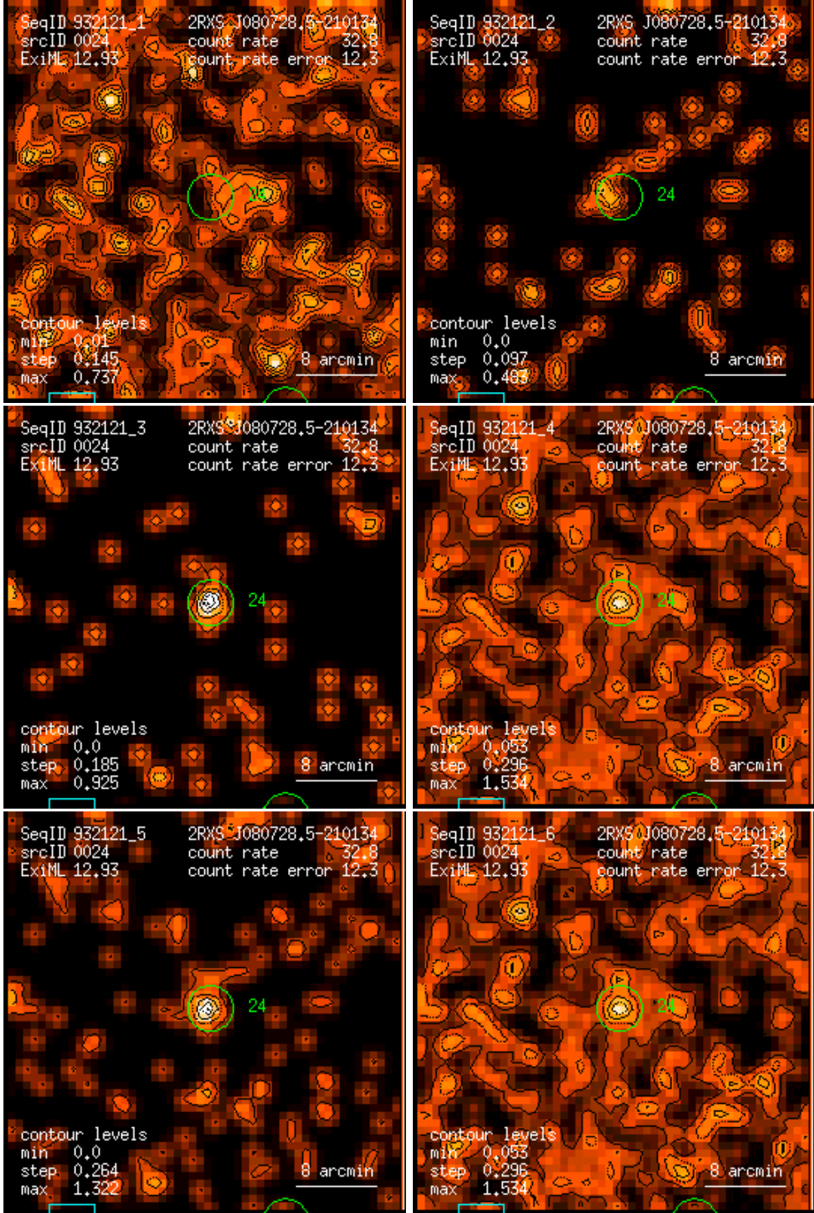
Figure 24: RASS 932121: detection 0024: band rate images, Gaussian filter: (1) PSPC channels 11 – 41, (2) 52 – 90, (3) 91 – 201, (4) 11 – 235, (5) 52 – 201, (6) 11 – 201. Broad band rates in counts/ks. Band rate contour levels in counts/ks/arcmin 2 .
