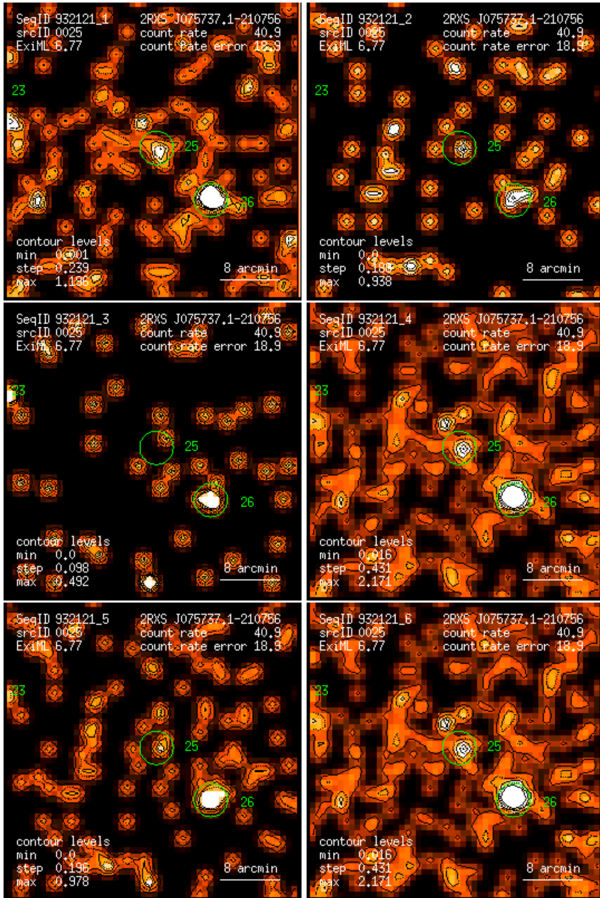
Figure 25: RASS 932121: detection 0025: band rate images, Gaussian filter: (1) PSPC channels 11 – 41, (2) 52 – 90, (3) 91 – 201, (4) 11 – 235, (5) 52 – 201, (6) 11 – 201. Broad band rates in counts/ks. Band rate contour levels in counts/ks/arcmin 2 .
