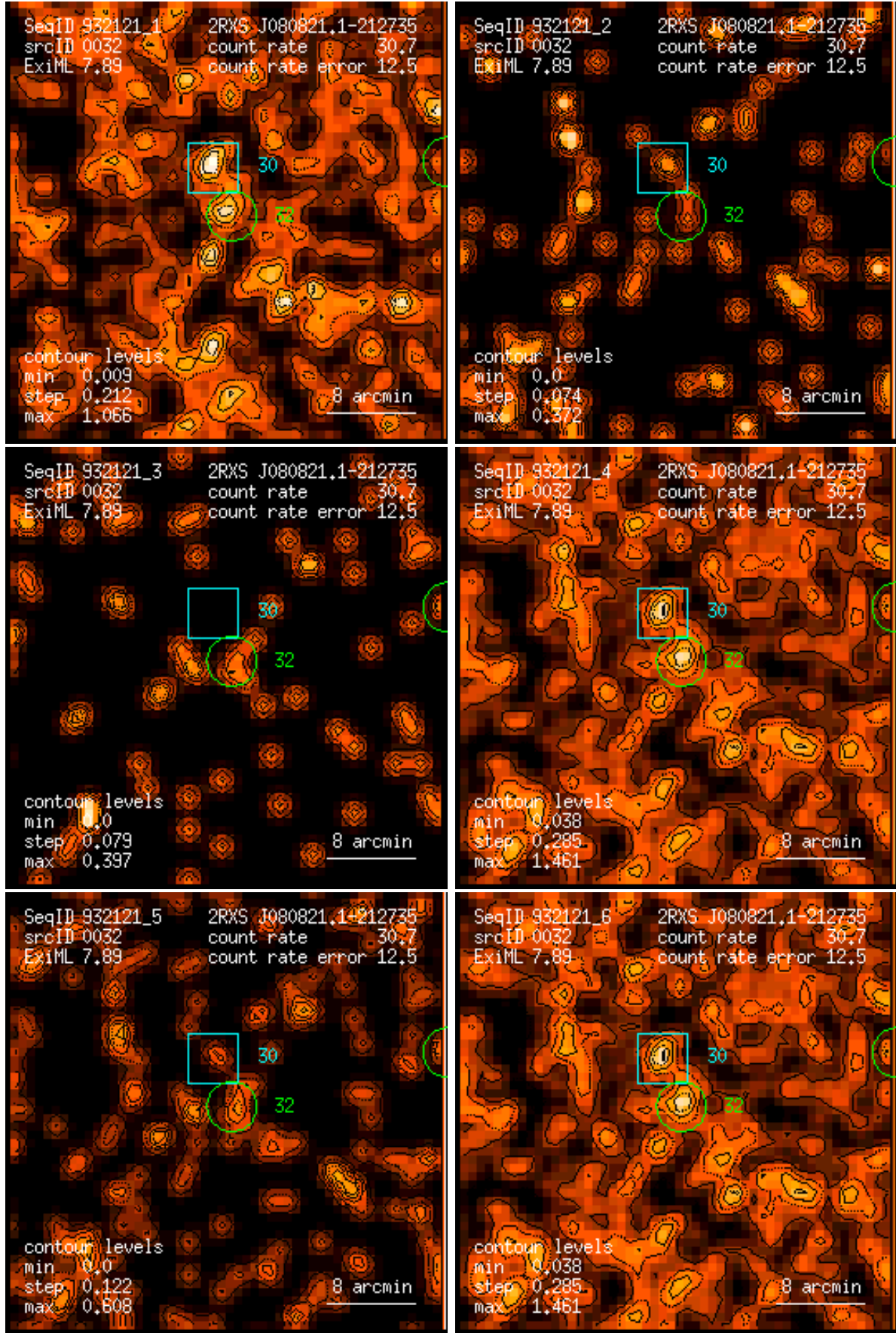
Figure 32: RASS 932121: detection 0032: band rate images, Gaussian filter: (1) PSPC channels 11 – 41, (2) 52 – 90, (3) 91 – 201, (4) 11 – 235, (5) 52 – 201, (6) 11 – 201. Broad band rates in counts/ks. Band rate contour levels in counts/ks/arcmin 2 .
