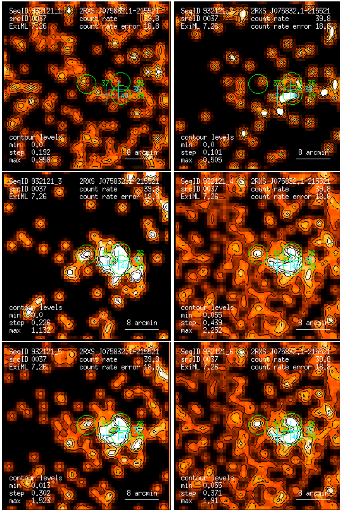
Figure 37: RASS 932121: detection 0037: band rate images, Gaussian filter: (1) PSPC channels 11 – 41, (2) 52 – 90, (3) 91 – 201, (4) 11 – 235, (5) 52 – 201, (6) 11 – 201. Broad band rates in counts/ks. Band rate contour levels in counts/ks/arcmin 2 .
