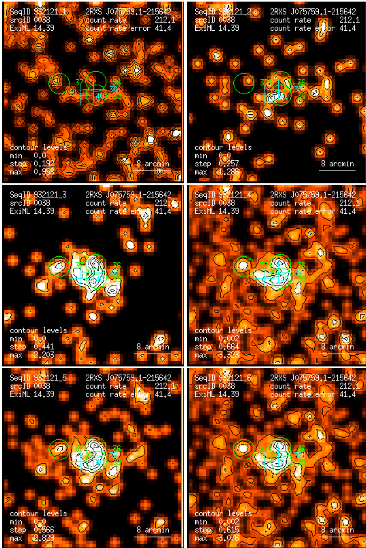
Figure 38: RASS 932121: detection 0038: band rate images, Gaussian filter: (1) PSPC channels 11 – 41, (2) 52 – 90, (3) 91 – 201, (4) 11 – 235, (5) 52 – 201, (6) 11 – 201. Broad band rates in counts/ks. Band rate contour levels in counts/ks/arcmin 2 .
