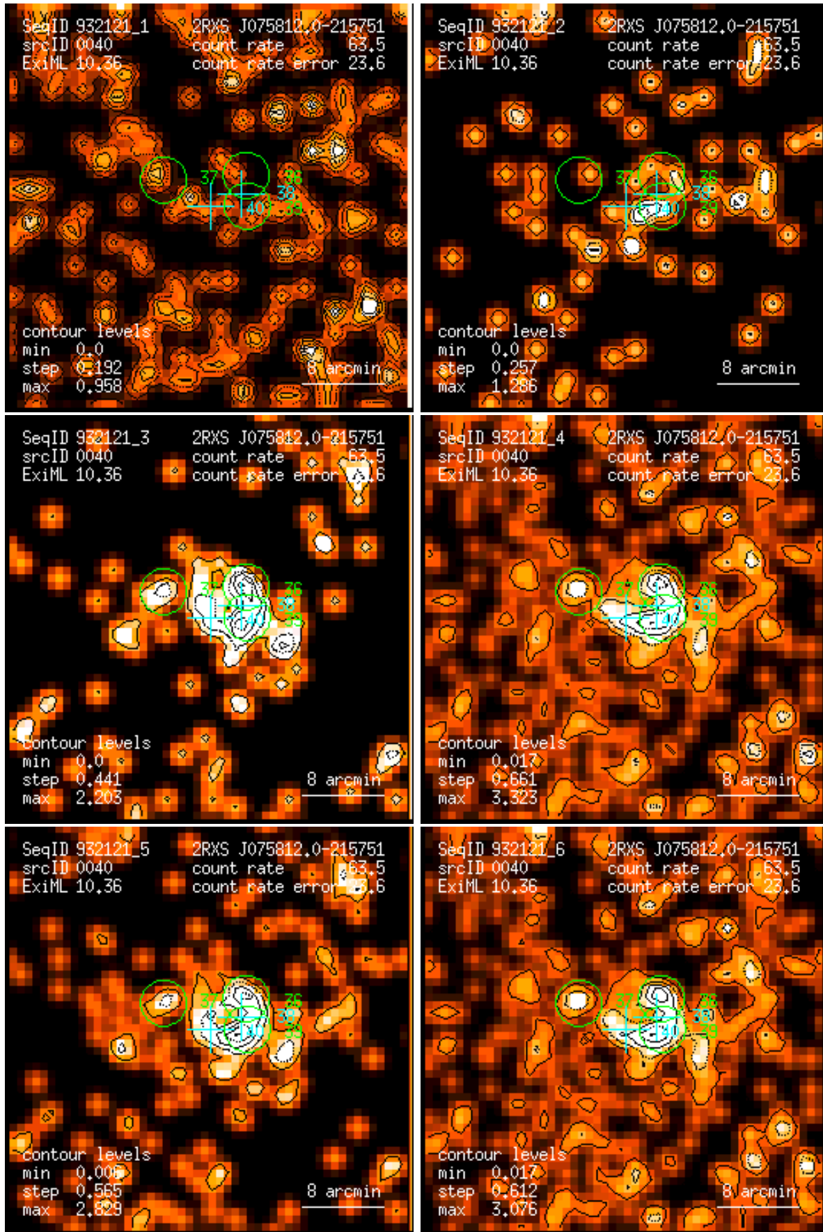
Figure 40: RASS 932121: detection 0040: band rate images, Gaussian filter: (1) PSPC channels 11 – 41, (2) 52 – 90, (3) 91 – 201, (4) 11 – 235, (5) 52 – 201, (6) 11 – 201. Broad band rates in counts/ks. Band rate contour levels in counts/ks/arcmin 2 .
