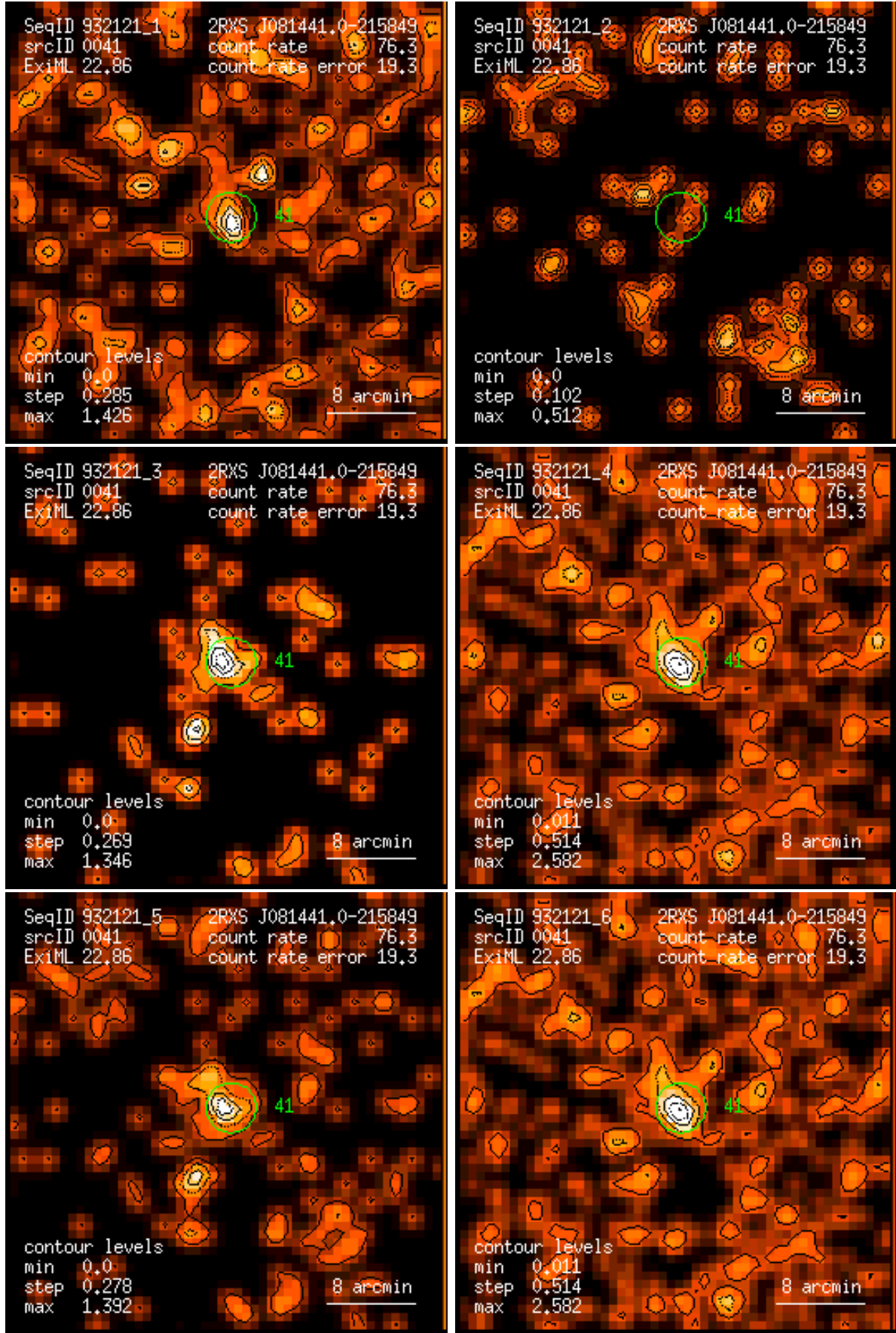
Figure 41: RASS 932121: detection 0041: band rate images, Gaussian filter: (1) PSPC channels 11 – 41, (2) 52 – 90, (3) 91 – 201, (4) 11 – 235, (5) 52 – 201, (6) 11 – 201. Broad band rates in counts/ks. Band rate contour levels in counts/ks/arcmin 2 .
