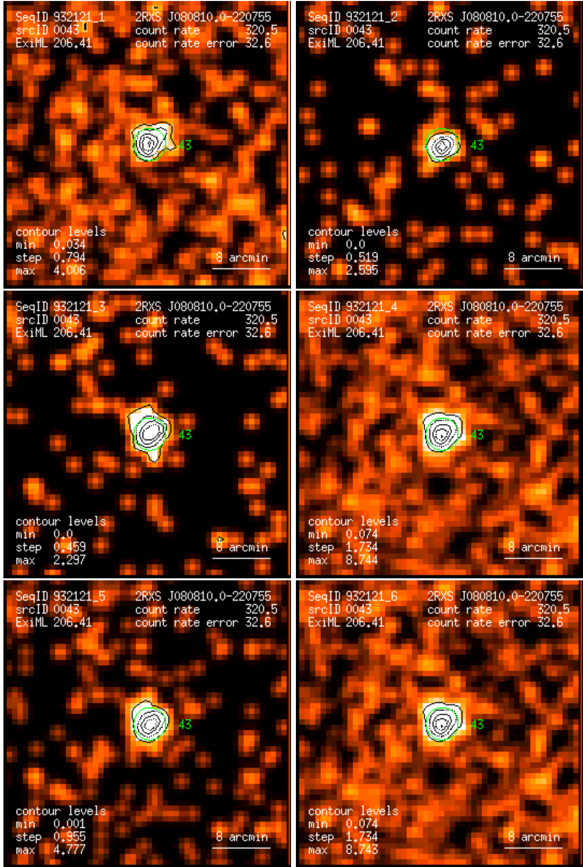
Figure 43: RASS 932121: detection 0043: band rate images, Gaussian filter: (1) PSPC channels 11 – 41, (2) 52 – 90, (3) 91 – 201, (4) 11 – 235, (5) 52 – 201, (6) 11 – 201. Broad band rates in counts/ks. Band rate contour levels in counts/ks/arcmin 2 .
