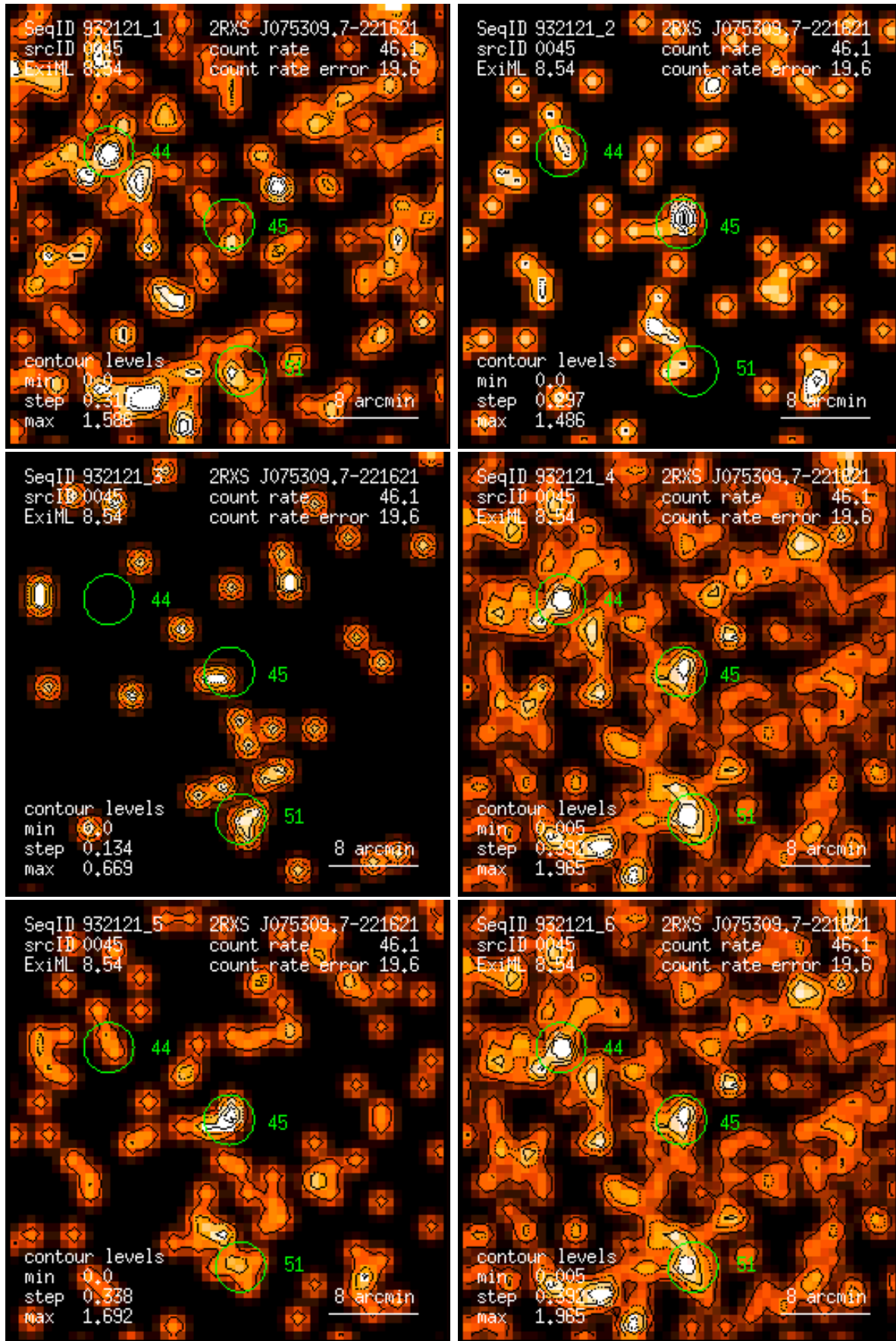
Figure 45: RASS 932121: detection 0045: band rate images, Gaussian filter: (1) PSPC channels 11 – 41, (2) 52 – 90, (3) 91 – 201, (4) 11 – 235, (5) 52 – 201, (6) 11 – 201. Broad band rates in counts/ks. Band rate contour levels in counts/ks/arcmin 2 .
