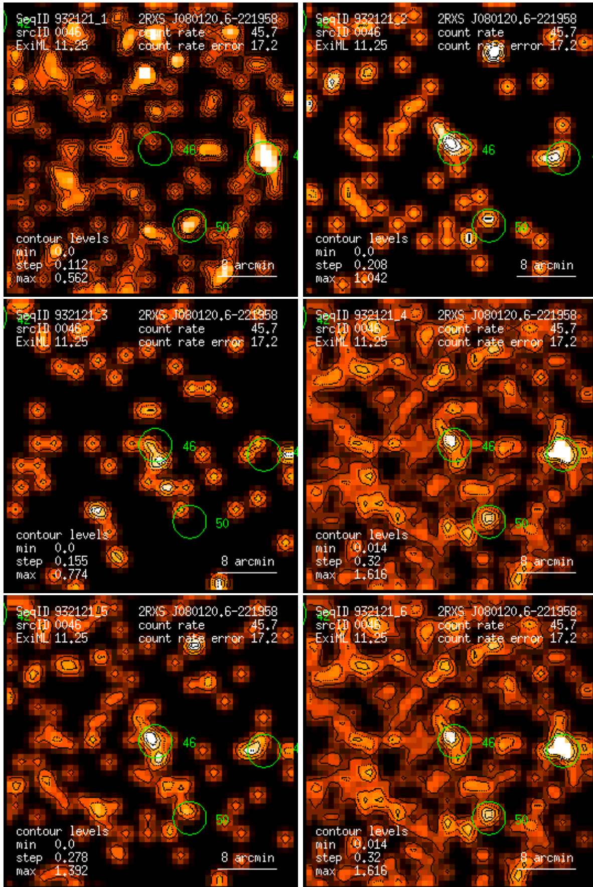
Figure 46: RASS 932121: detection 0046: band rate images, Gaussian filter: (1) PSPC channels 11 – 41, (2) 52 – 90, (3) 91 – 201, (4) 11 – 235, (5) 52 – 201, (6) 11 – 201. Broad band rates in counts/ks. Band rate contour levels in counts/ks/arcmin 2 .
