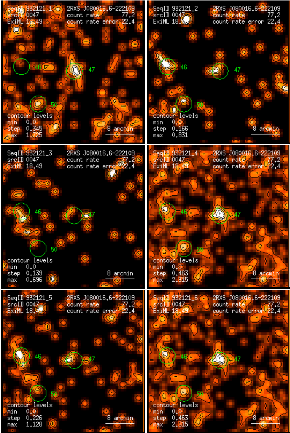
Figure 47: RASS 932121: detection 0047: band rate images, Gaussian filter: (1) PSPC channels 11 – 41, (2) 52 – 90, (3) 91 – 201, (4) 11 – 235, (5) 52 – 201, (6) 11 – 201. Broad band rates in counts/ks. Band rate contour levels in counts/ks/arcmin 2 .
