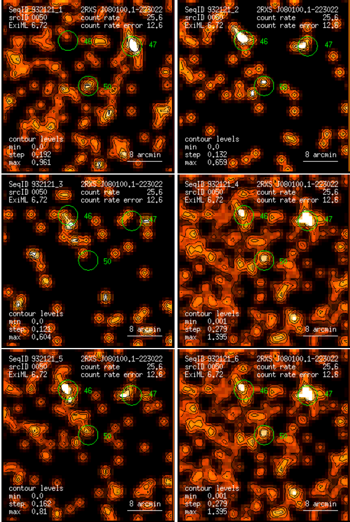
Figure 50: RASS 932121: detection 0050: band rate images, Gaussian filter: (1) PSPC channels 11 – 41, (2) 52 – 90, (3) 91 – 201, (4) 11 – 235, (5) 52 – 201, (6) 11 – 201. Broad band rates in counts/ks. Band rate contour levels in counts/ks/arcmin 2 .
