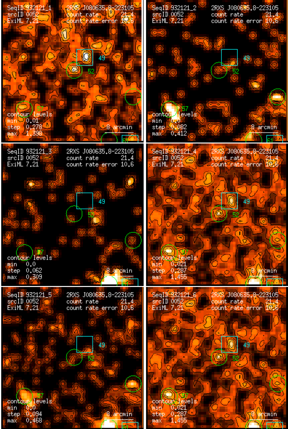
Figure 52: RASS 932121: detection 0052: band rate images, Gaussian filter: (1) PSPC channels 11 – 41, (2) 52 – 90, (3) 91 – 201, (4) 11 – 235, (5) 52 – 201, (6) 11 – 201. Broad band rates in counts/ks. Band rate contour levels in counts/ks/arcmin 2 .
