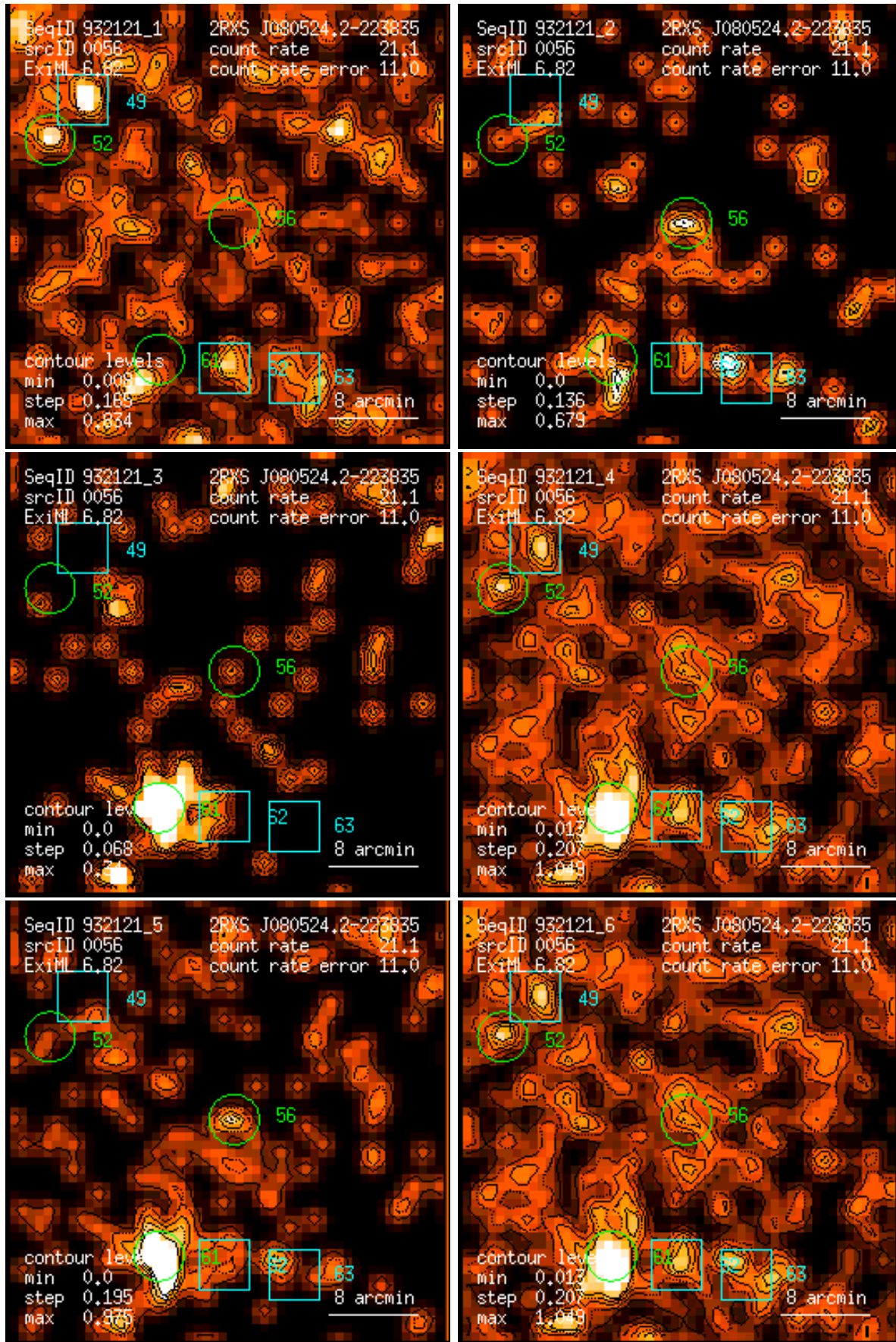
Figure 56: RASS 932121: detection 0056: band rate images, Gaussian filter: (1) PSPC channels 11 – 41, (2) 52 – 90, (3) 91 – 201, (4) 11 – 235, (5) 52 – 201, (6) 11 – 201. Broad band rates in counts/ks. Band rate contour levels in counts/ks/arcmin 2 .
