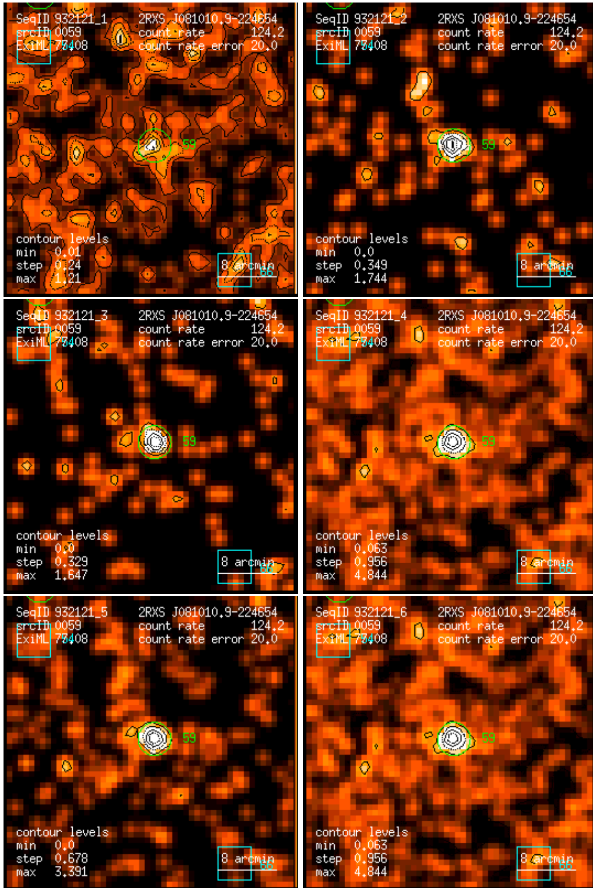
Figure 59: RASS 932121: detection 0059: band rate images, Gaussian filter: (1) PSPC channels 11 – 41, (2) 52 – 90, (3) 91 – 201, (4) 11 – 235, (5) 52 – 201, (6) 11 – 201. Broad band rates in counts/ks. Band rate contour levels in counts/ks/arcmin 2 .
