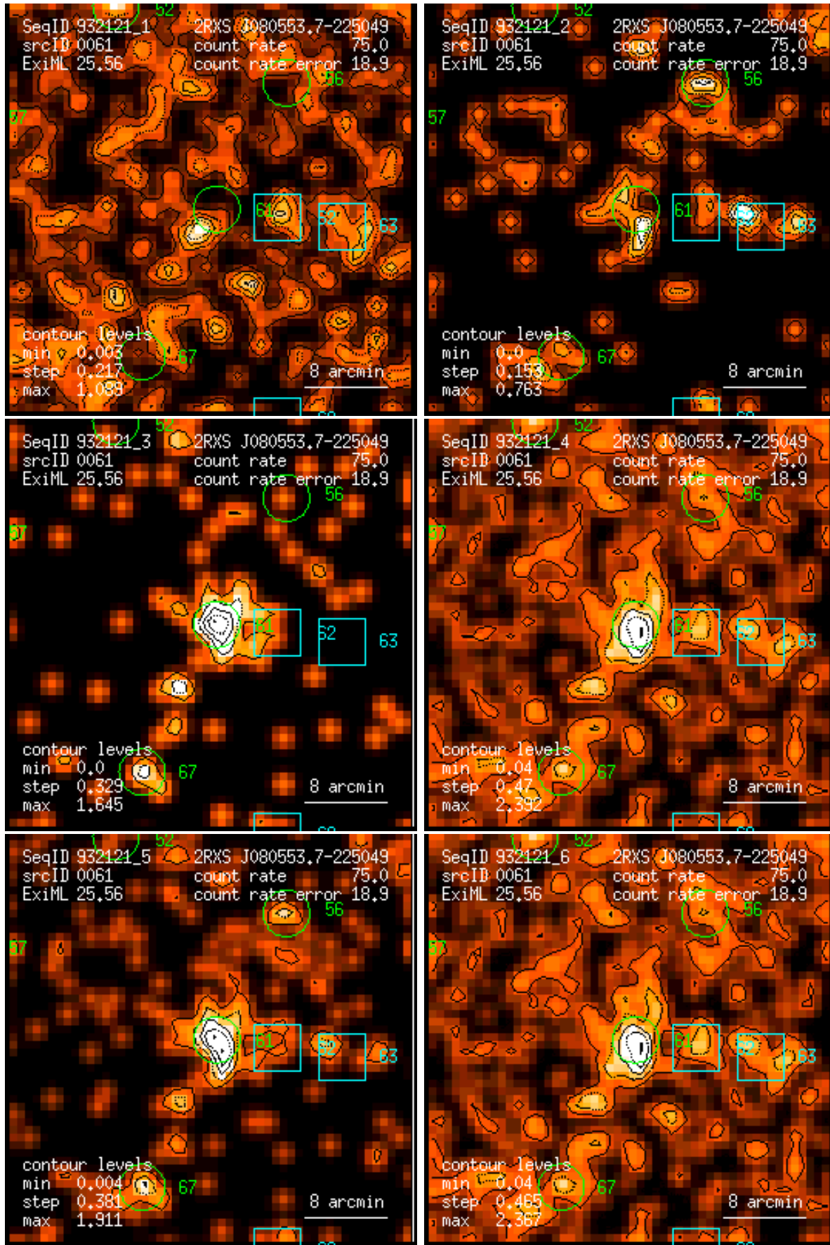
Figure 61: RASS 932121: detection 0061: band rate images, Gaussian filter: (1) PSPC channels 11 – 41, (2) 52 – 90, (3) 91 – 201, (4) 11 – 235, (5) 52 – 201, (6) 11 – 201. Broad band rates in counts/ks. Band rate contour levels in counts/ks/arcmin 2 .
