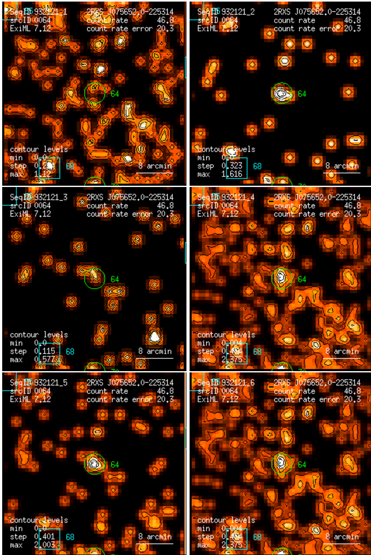
Figure 64: RASS 932121: detection 0064: band rate images, Gaussian filter: (1) PSPC channels 11 – 41, (2) 52 – 90, (3) 91 – 201, (4) 11 – 235, (5) 52 – 201, (6) 11 – 201. Broad band rates in counts/ks. Band rate contour levels in counts/ks/arcmin 2 .
