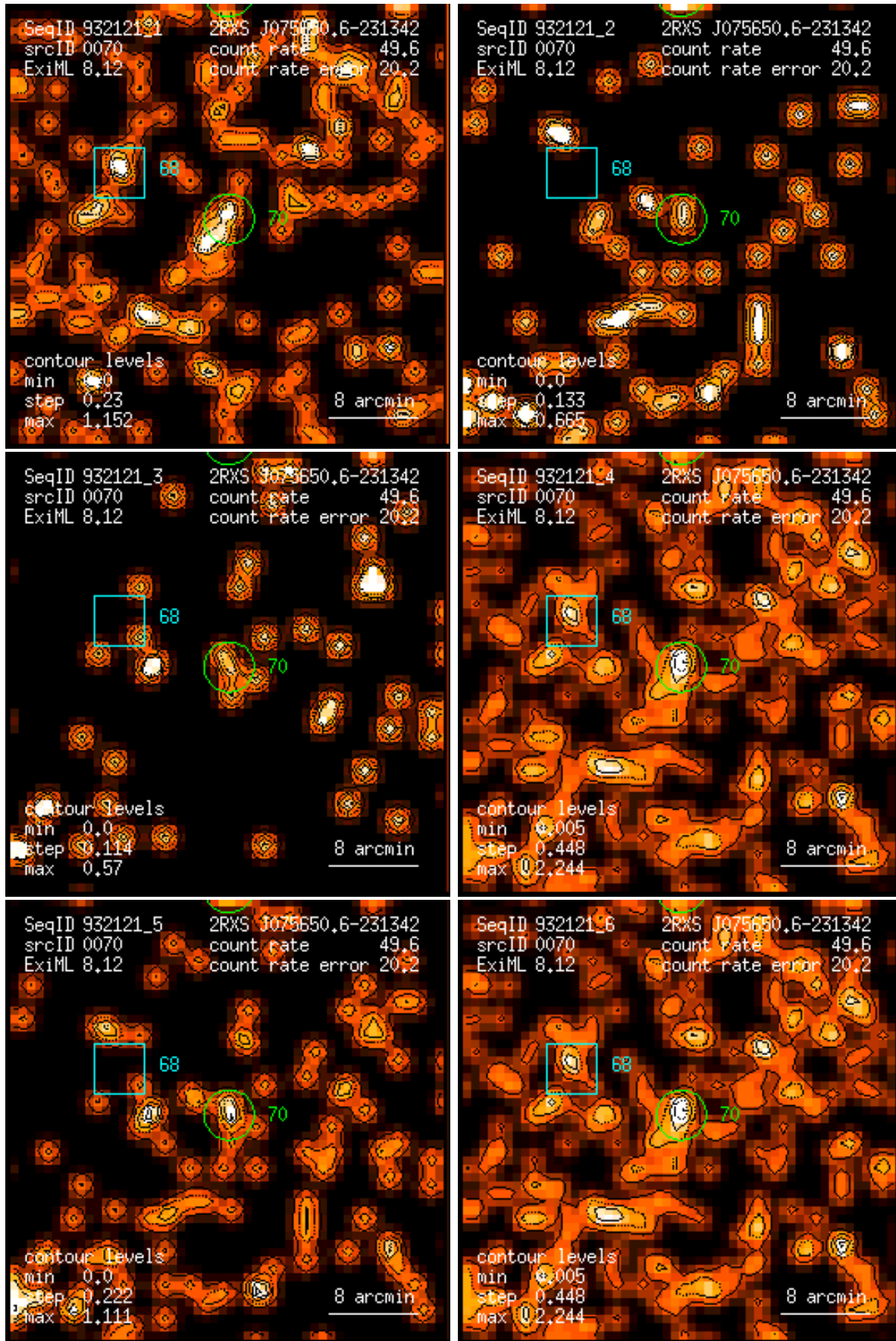
Figure 70: RASS 932121: detection 0070: band rate images, Gaussian filter: (1) PSPC channels 11 – 41, (2) 52 – 90, (3) 91 – 201, (4) 11 – 235, (5) 52 – 201, (6) 11 – 201. Broad band rates in counts/ks. Band rate contour levels in counts/ks/arcmin 2 .
