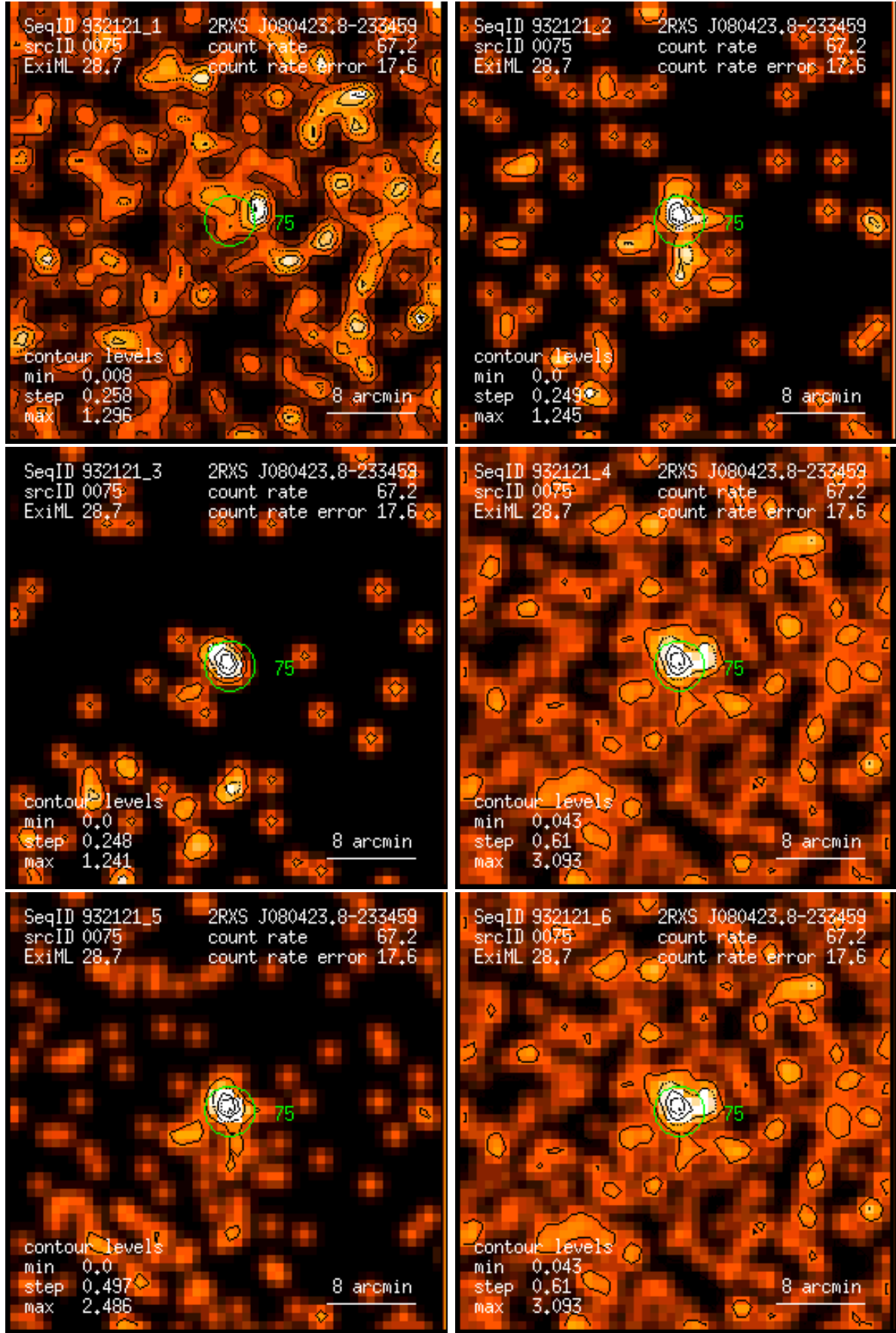
Figure 75: RASS 932121: detection 0075: band rate images, Gaussian filter: (1) PSPC channels 11 – 41, (2) 52 – 90, (3) 91 – 201, (4) 11 – 235, (5) 52 – 201, (6) 11 – 201. Broad band rates in counts/ks. Band rate contour levels in counts/ks/arcmin 2 .
