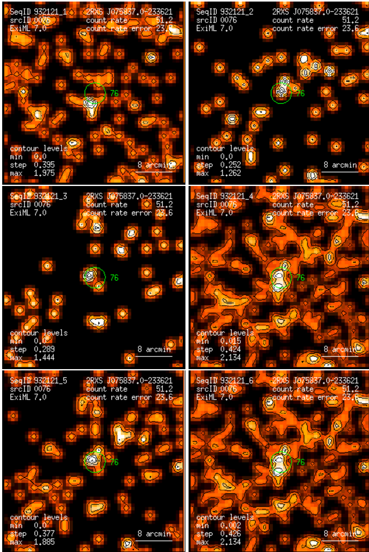
Figure 76: RASS 932121: detection 0076: band rate images, Gaussian filter: (1) PSPC channels 11 – 41, (2) 52 – 90, (3) 91 – 201, (4) 11 – 235, (5) 52 – 201, (6) 11 – 201. Broad band rates in counts/ks. Band rate contour levels in counts/ks/arcmin 2 .
