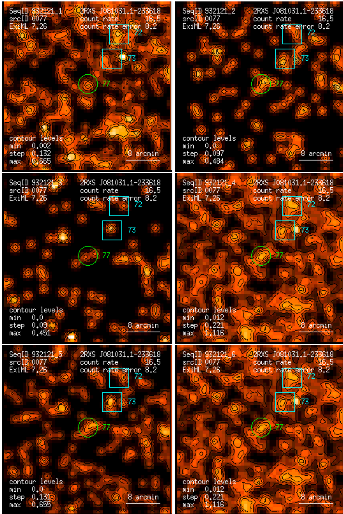
Figure 77: RASS 932121: detection 0077: band rate images, Gaussian filter: (1) PSPC channels 11 – 41, (2) 52 – 90, (3) 91 – 201, (4) 11 – 235, (5) 52 – 201, (6) 11 – 201. Broad band rates in counts/ks. Band rate contour levels in counts/ks/arcmin 2 .
