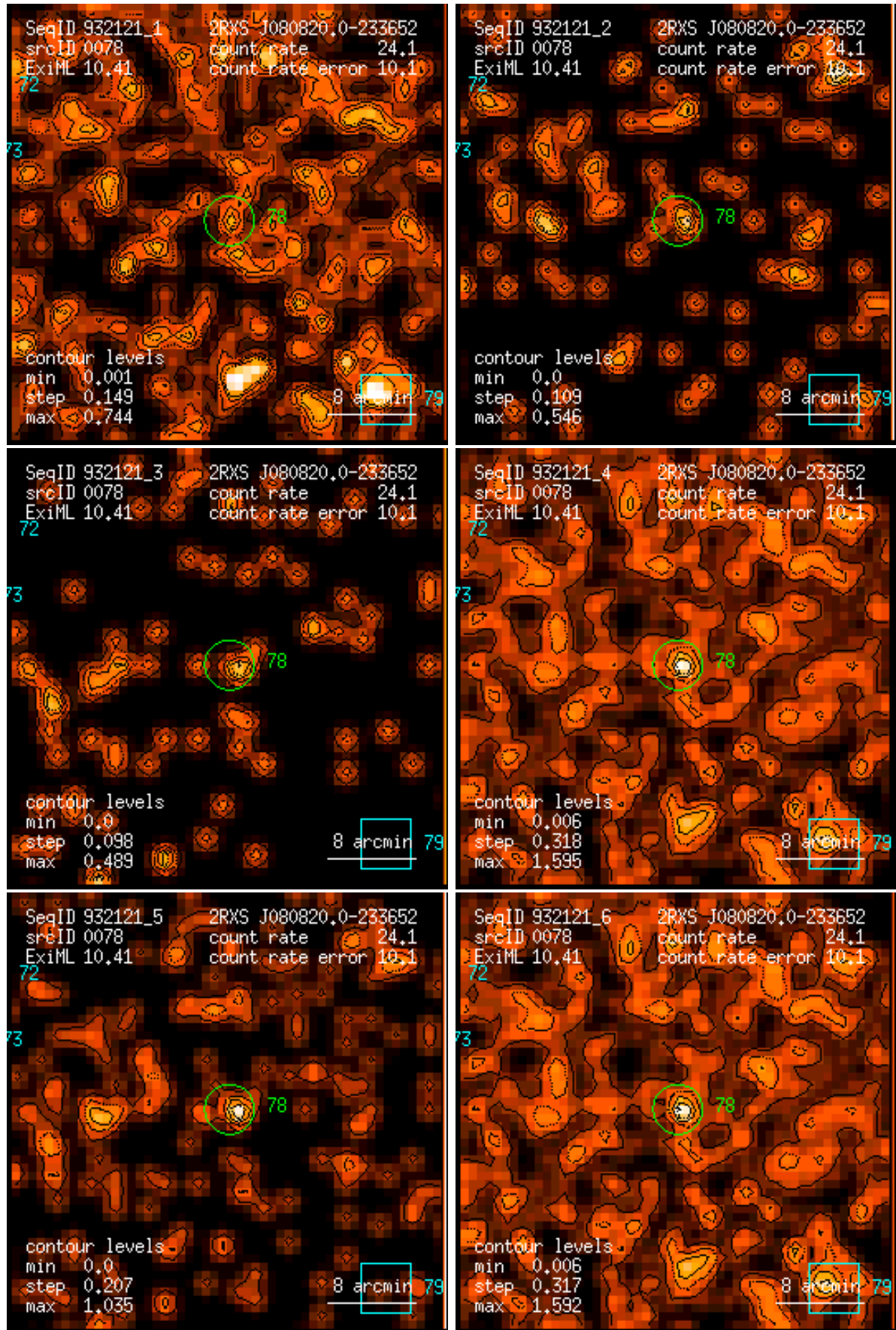
Figure 78: RASS 932121: detection 0078: band rate images, Gaussian filter: (1) PSPC channels 11 – 41, (2) 52 – 90, (3) 91 – 201, (4) 11 – 235, (5) 52 – 201, (6) 11 – 201. Broad band rates in counts/ks. Band rate contour levels in counts/ks/arcmin 2 .
